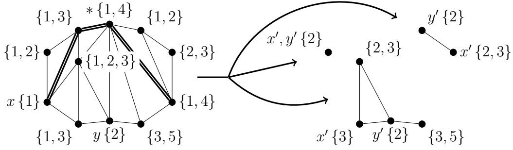
Figure 6: Coloring and removing a path P in Hartman's proof of [7, Lemma. 4.2].
