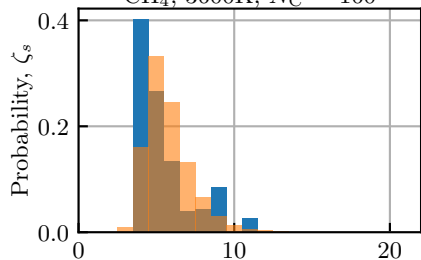
\text{CH}_4 , 3600K, N_C = 160
