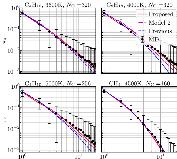
(a) Molecule Size: #C atoms (s) Molecule Size: #C atoms (s)
