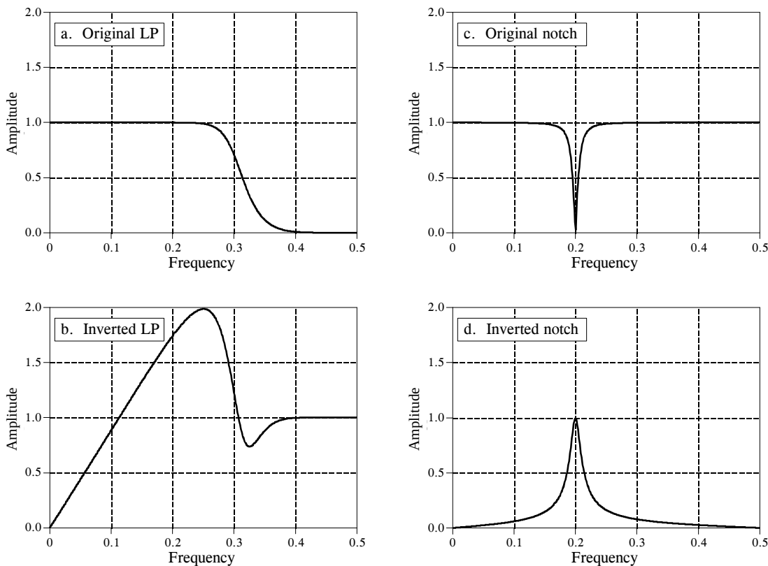
FIGURE 33-6 Examples of spectral inversion. Figure (a) shows the frequency response of a 6 pole low-pass Butterworth filter. Figure (b) shows the corresponding high-pass filter obtained by spectral inversion; its a mess! A more successful case is shown in (c) and (d) where a notch filter is transformed in to a band-pass frequency response.
