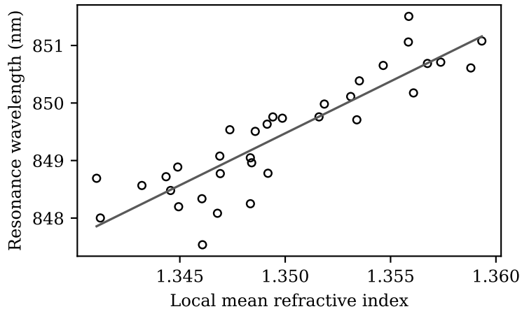
(a) 34 tissue realizations slope 181 nm/RIU
