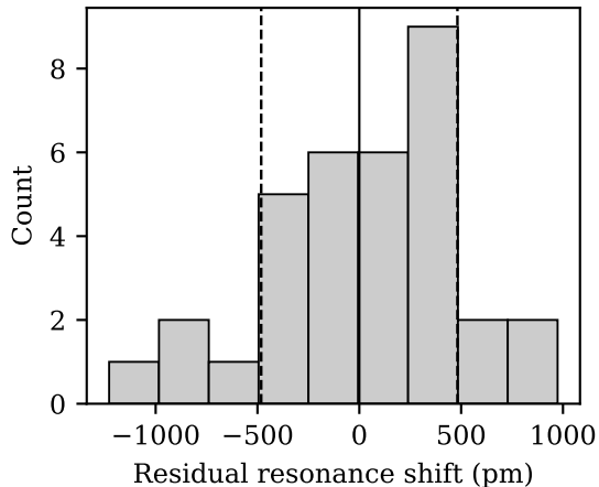
(b) After removing bulk drift \sigma = 482 pm
