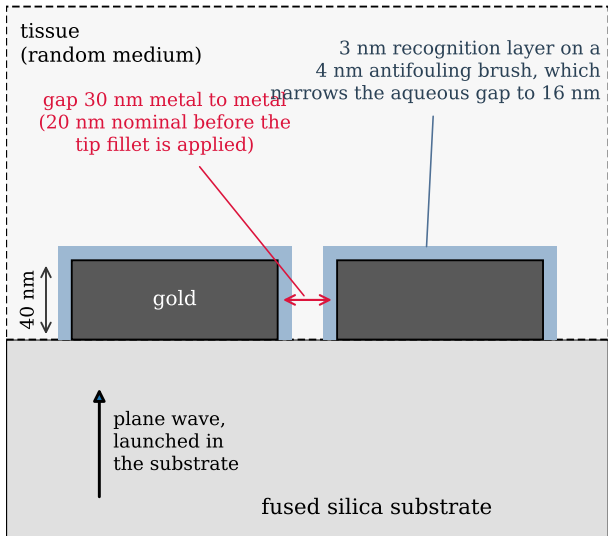
(a) Simulation geometry, side view
