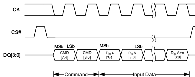
Figure 29. QPI SDR Transaction with Command and Data Input
