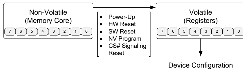
Figure 68. Data Movement Within Register Components
