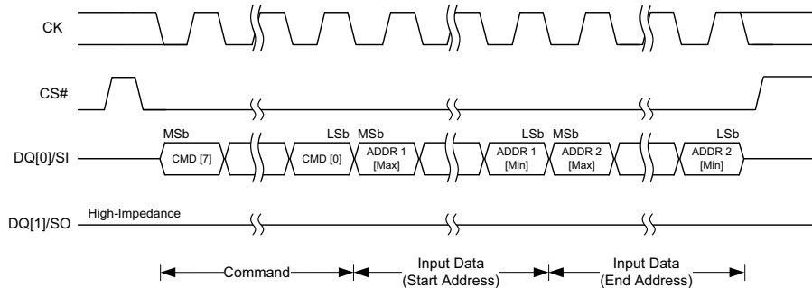
Figure 9. SPI Transaction with Command and Two Input Addresses
