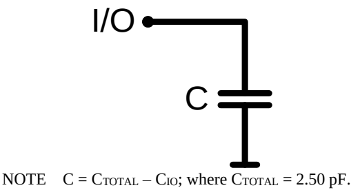
Figure 100 — Timing Reference Load
