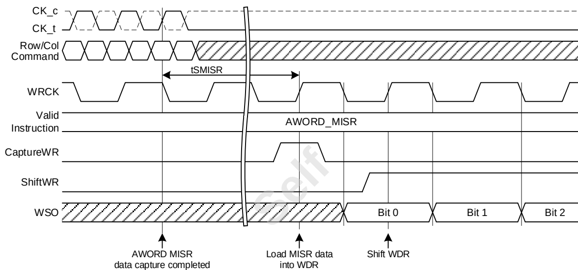
Figure 122 — IEEE1500 DWORD_MISR / AWORD_MISR Instruction Related Timings
