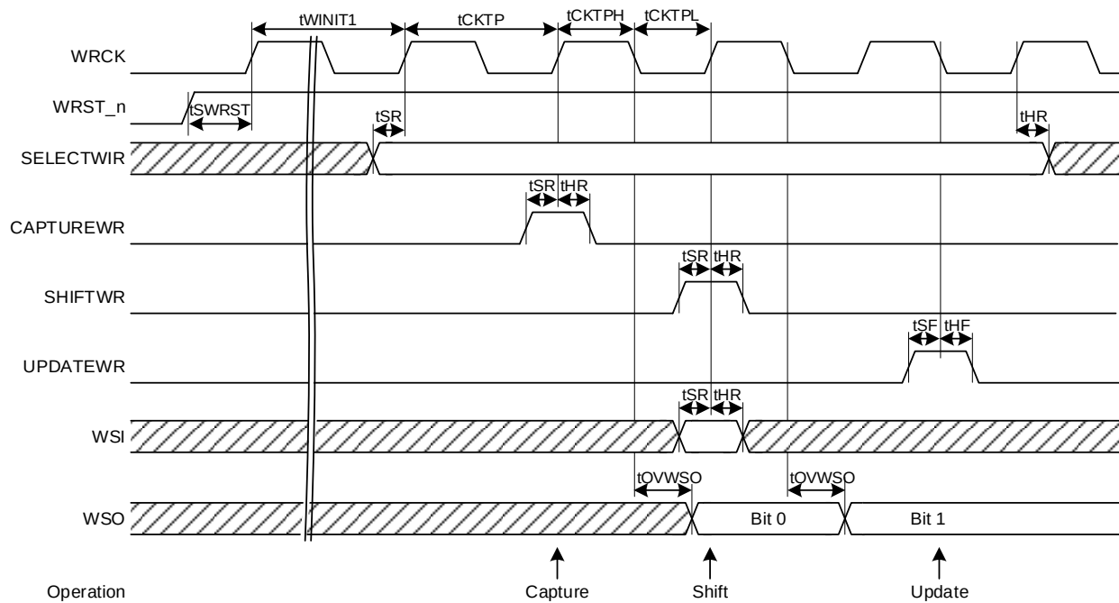
Figure 118 — IEEE1500 Port Input and Output Timings
