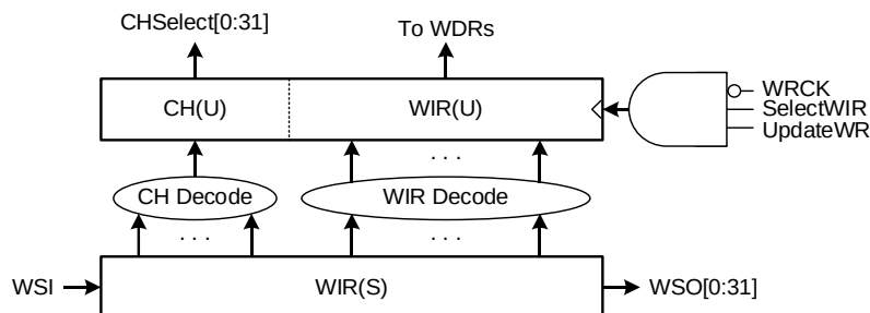
Figure 111 — WIR Channel Select Logic Diagram
