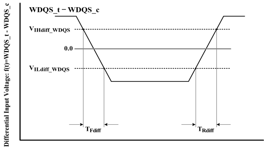
Figure 99 — Differential Input Slew Rate Definition for WDQS_t, WDQS_c
