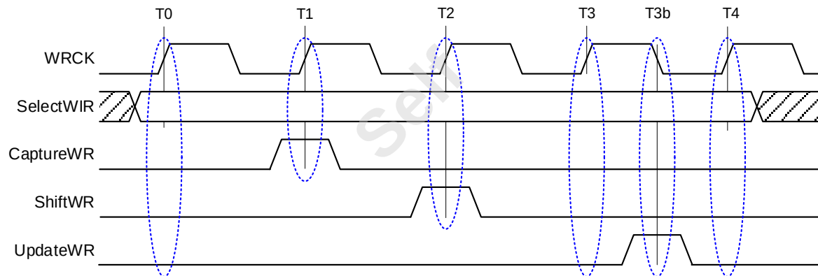
Figure 112 — IEEE1500 Port Operation
