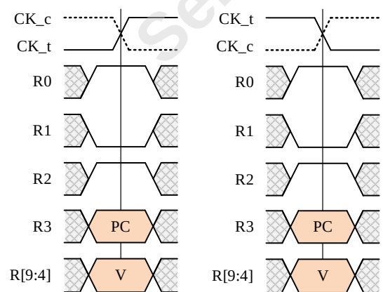
Figure 22 — PRECHARGE ALL (PREab) Command
