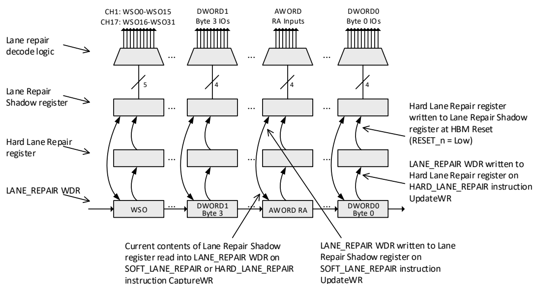
Figure 114 — Registers Associated with Lane Repair Instructions
