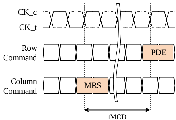
Figure 55 — MODE REGISTER SET to Power-Down Entry Timing
