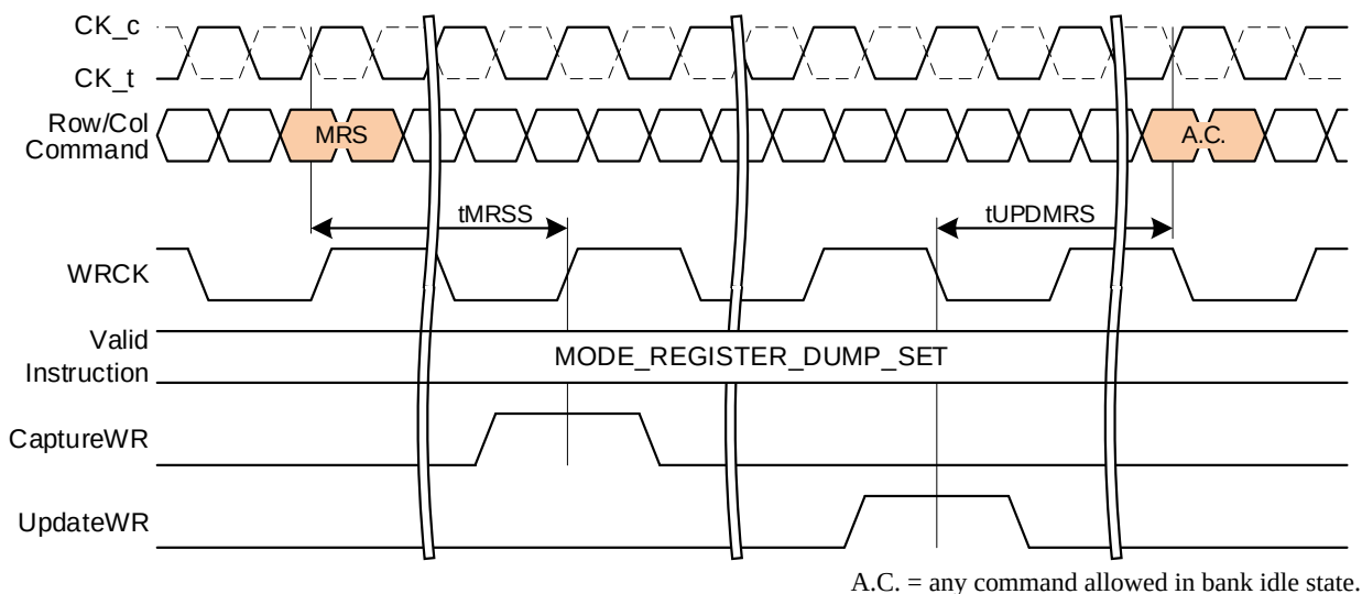
Figure 124 — IEEE1500 MODE_REGISTER_DUMP_SET Instruction Related Timings
