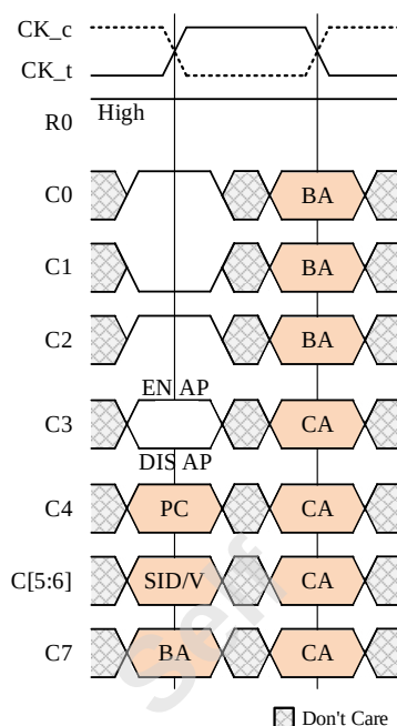
Figure 34 — READ Command
