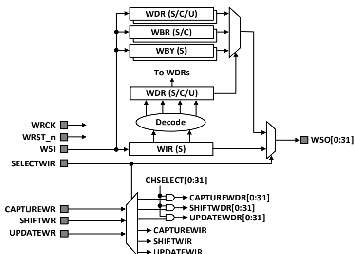
Figure 110 — IEEE Std. 1500 Logic Diagram
