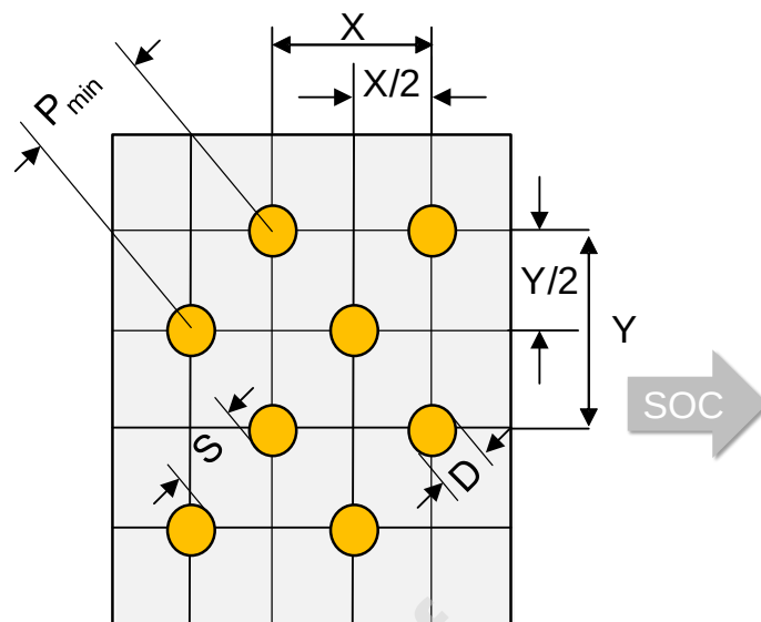
Figure 104 — Staggered MicroBump Pattern
