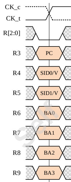
Figure 26 — REFRESH per-bank Command (REFpb)
