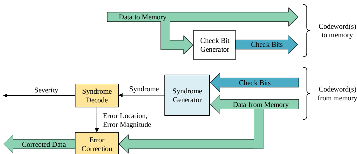
Figure 77 — On-die ECC Overview Diagram Example
