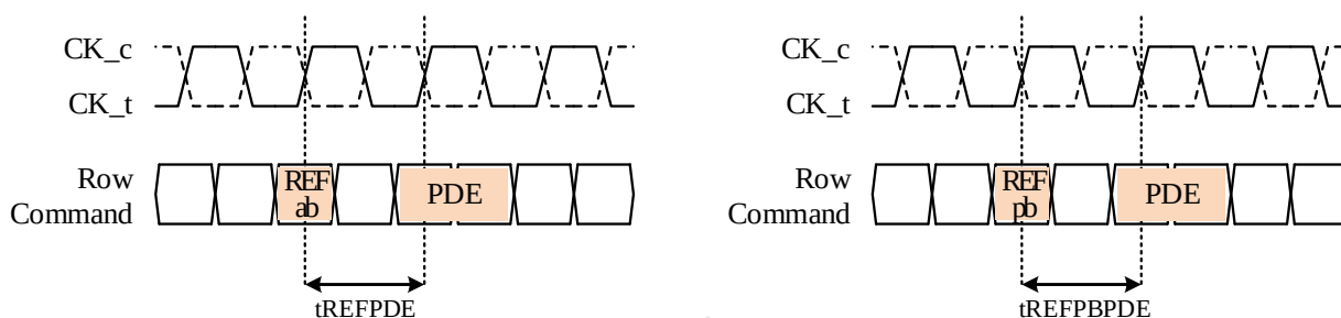
Figure 57 — REFab or REFpb to Power-Down Entry Timing
