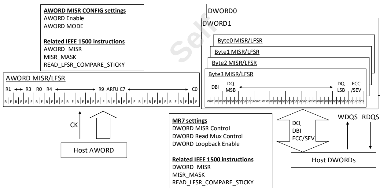
MISR Block Diagram
