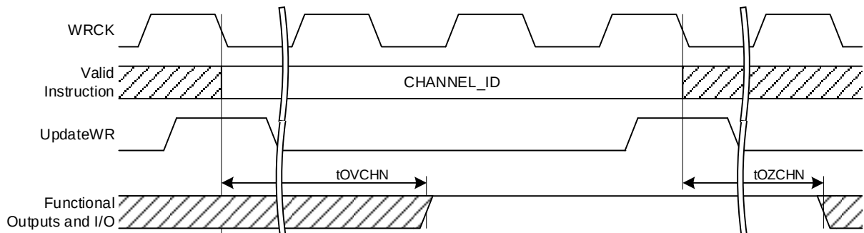
Figure 123 — IEEE1500 CHANNEL_ID Instruction Related Timings
