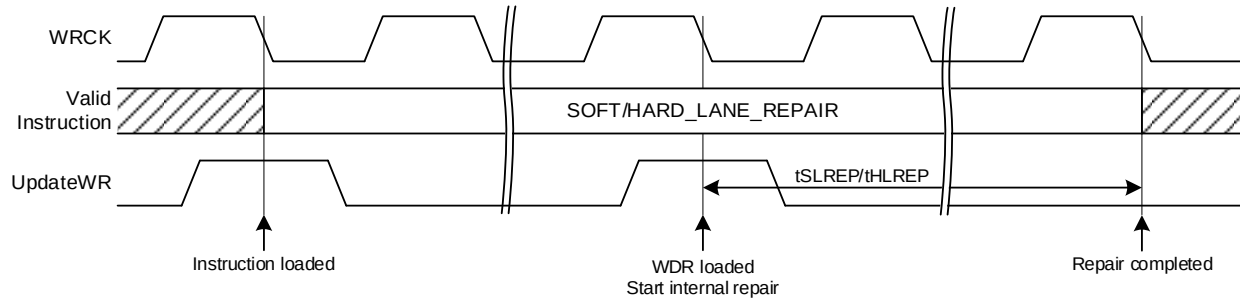
Figure 121 — IEEE1500 Soft_Lane_Repair and Hard_Lane_Repair Instruction Related Timings
