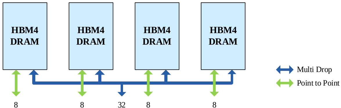
Figure 109 — DA Port Connection Diagram For Multiple HBM4 DRAM Devices
