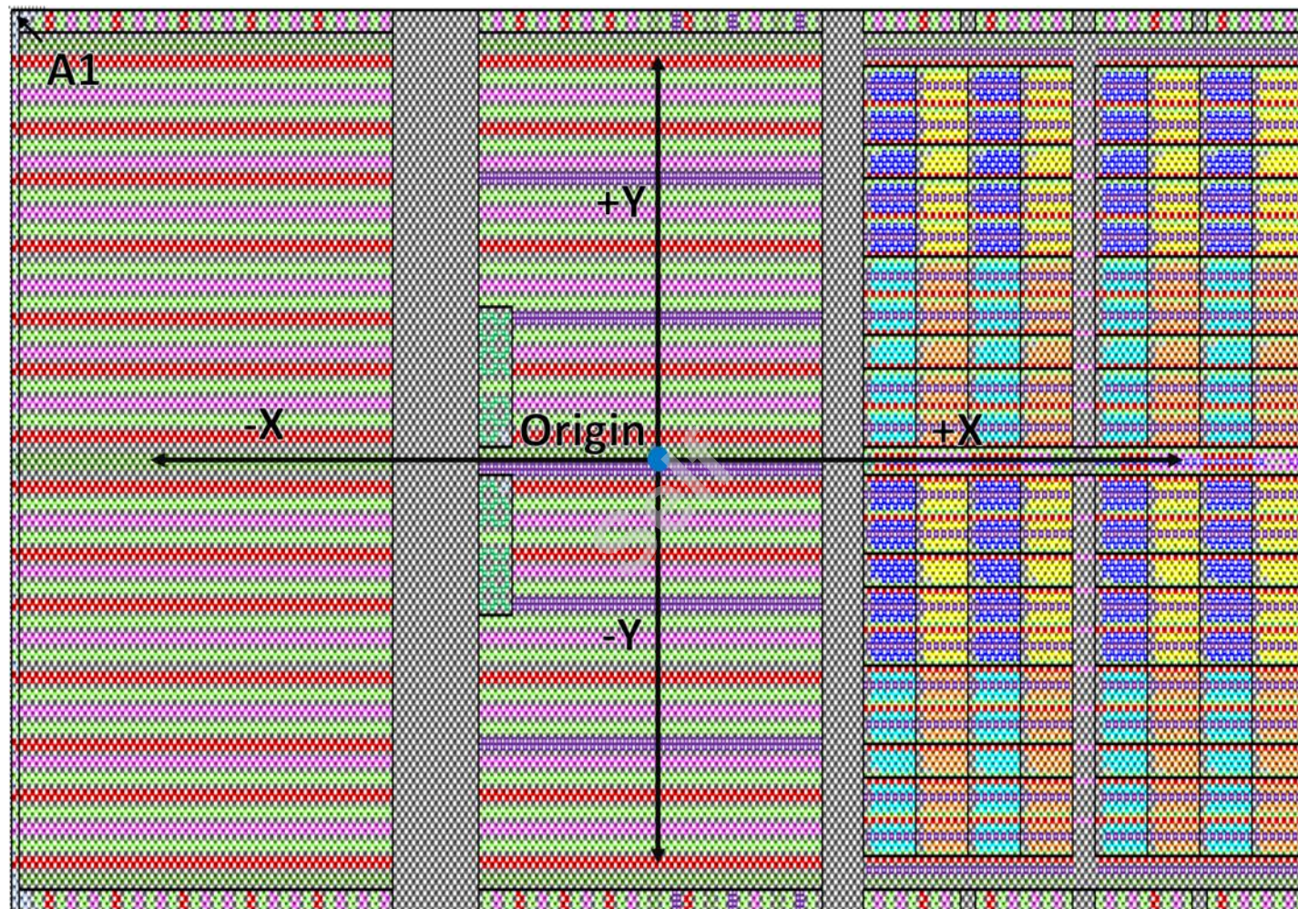
Figure 107 — Overview of HBM4 Bump Map Footprint B
