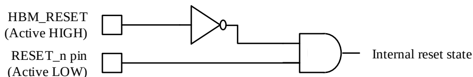
Figure 113 — RESET_n and HBM_RESET Logic
