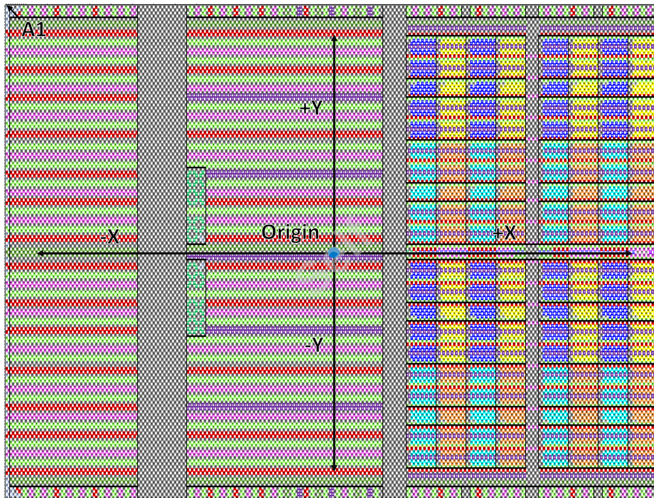
Figure 106 — Overview of HBM4 Bump Map Footprint A
