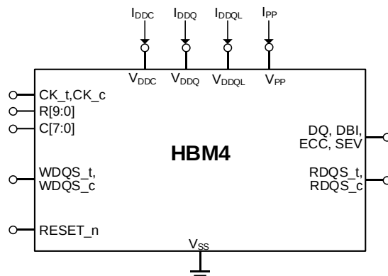
Figure 103 — Measurement Setup for IDD and IPP Measurements
