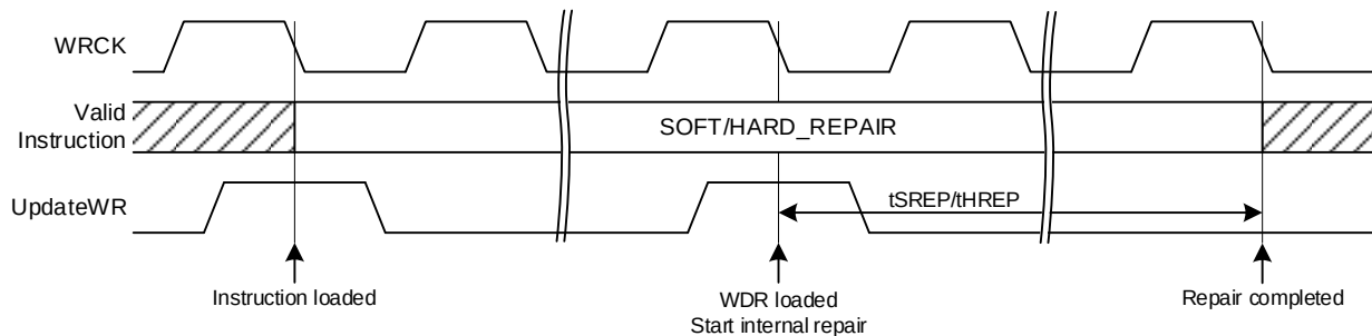
Figure 120 — IEEE1500 SOFT_REPAIR and HARD_REPAIR Instruction Related Timings
