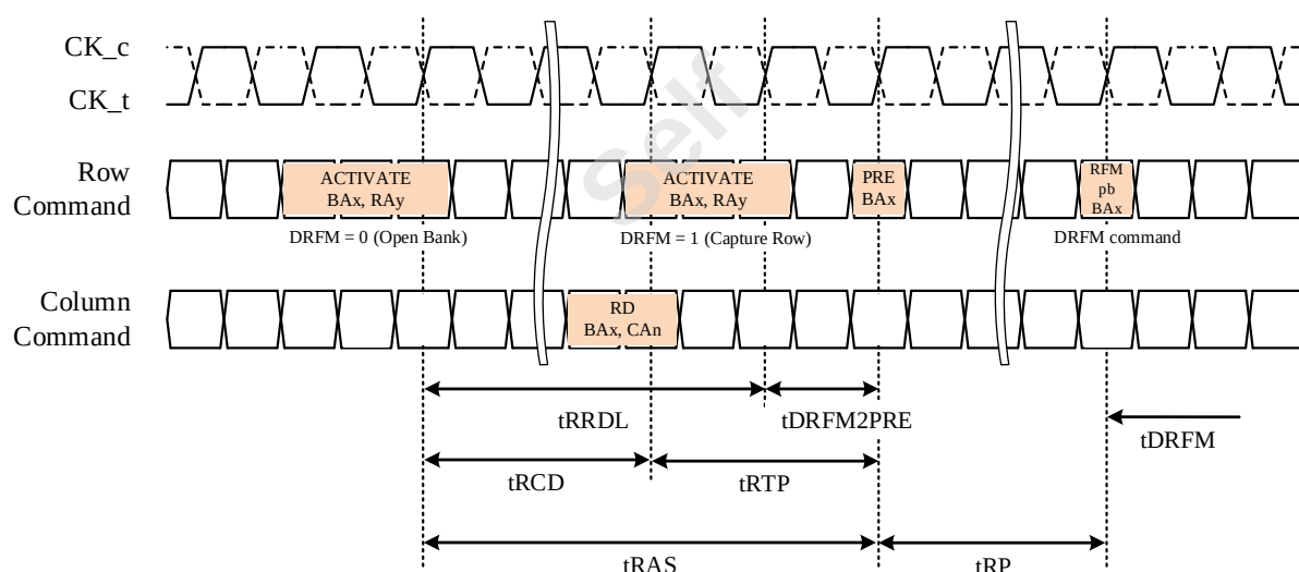
Figure 32 — ACTIVATE with DRFM Bit to Open Page (Same Bank and Row Address)
