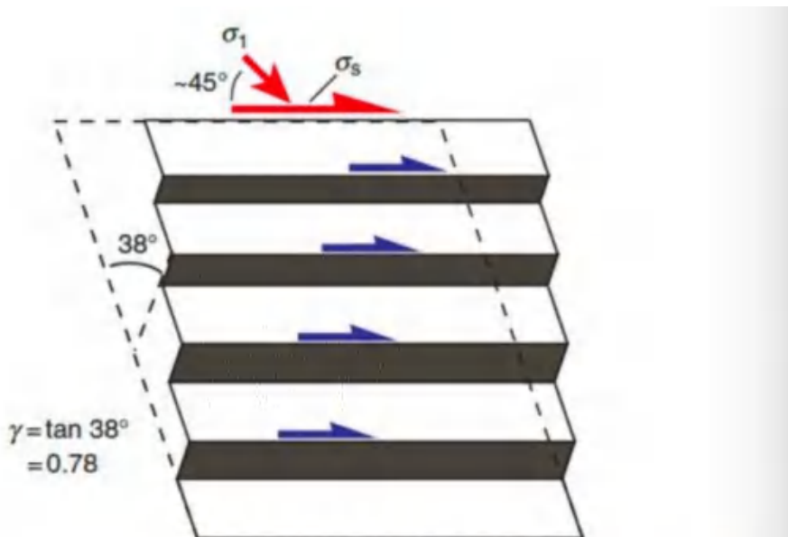
Figure 10.3 Deformation (glide) twins in a calcite crystal. Stress is ideally at 45^\circ to the shear (glide) plane. Dark lamellae have been sheared (simple shear).
