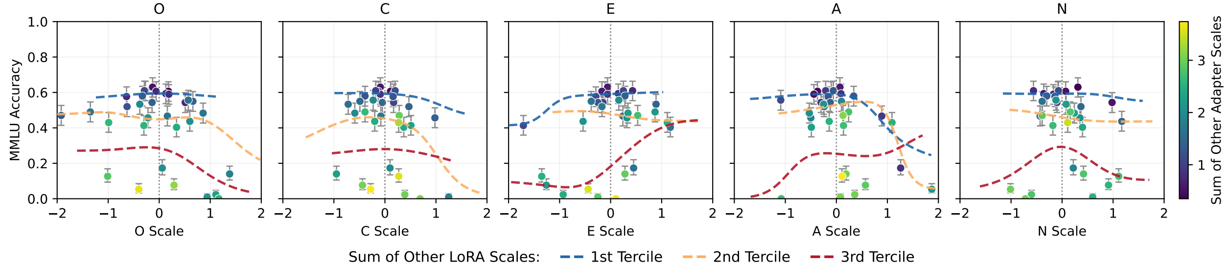
MMLU Scores vs Scales of Randomly Scaled OCEAN LoRA Combinations
