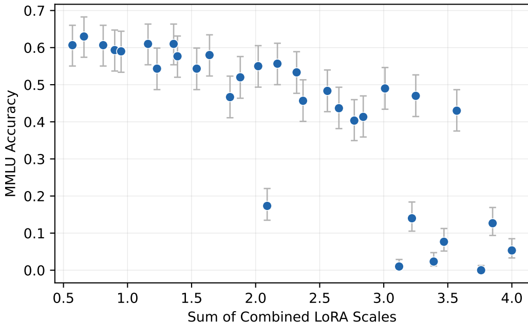
MMLU Accuracy vs Sum of Combined LoRA Scales for Randomly Scaled OCEAN LoRA Combinations
