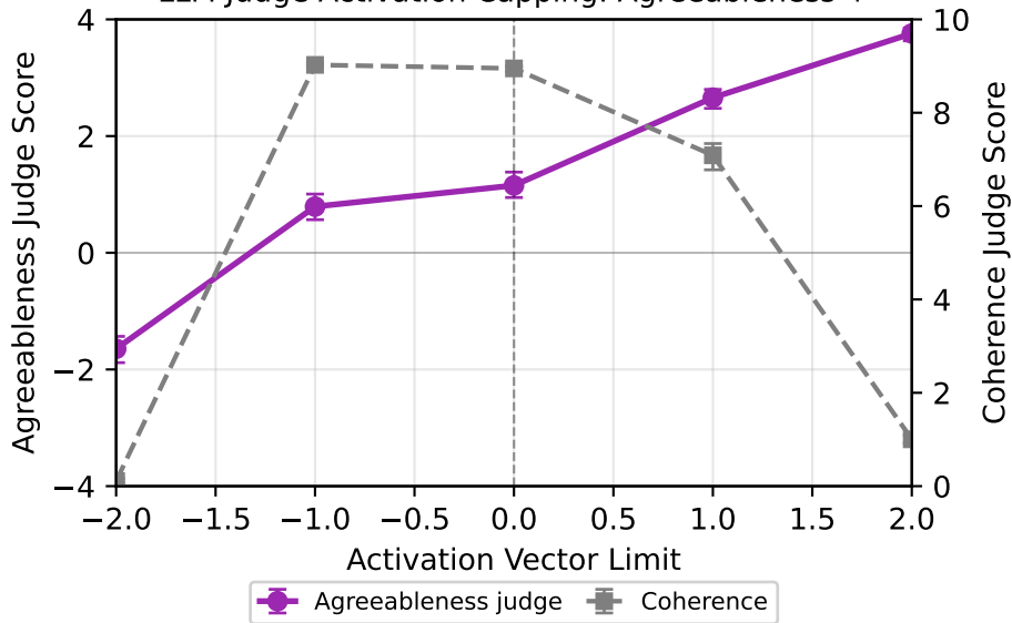
LLM Judge Activation Capping: Agreeableness \uparrow
