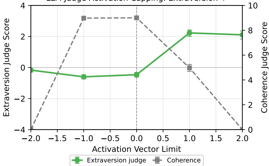
LLM Judge Activation Capping: Extraversion \uparrow
