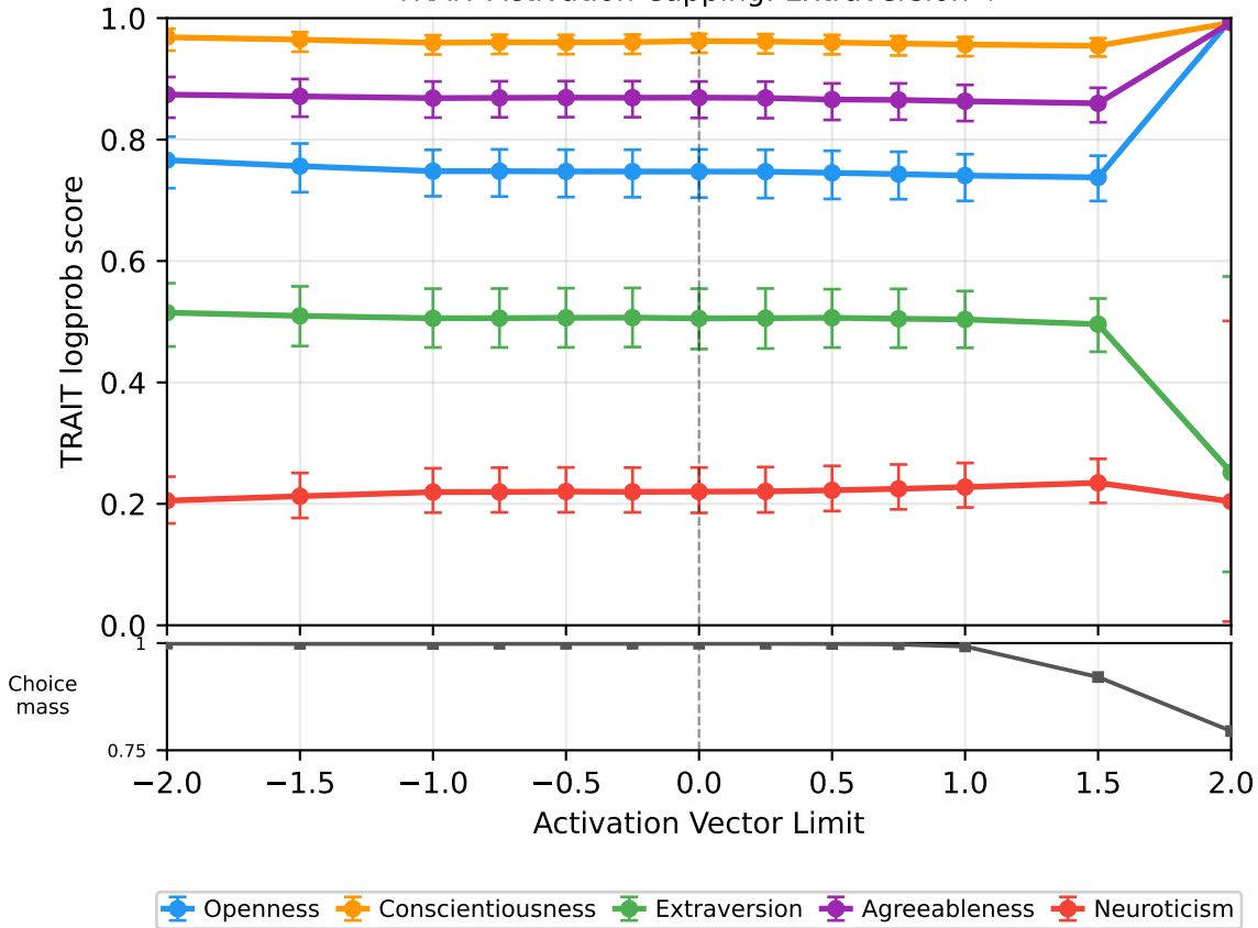
TRAIT Activation Capping: Extraversion ↓
