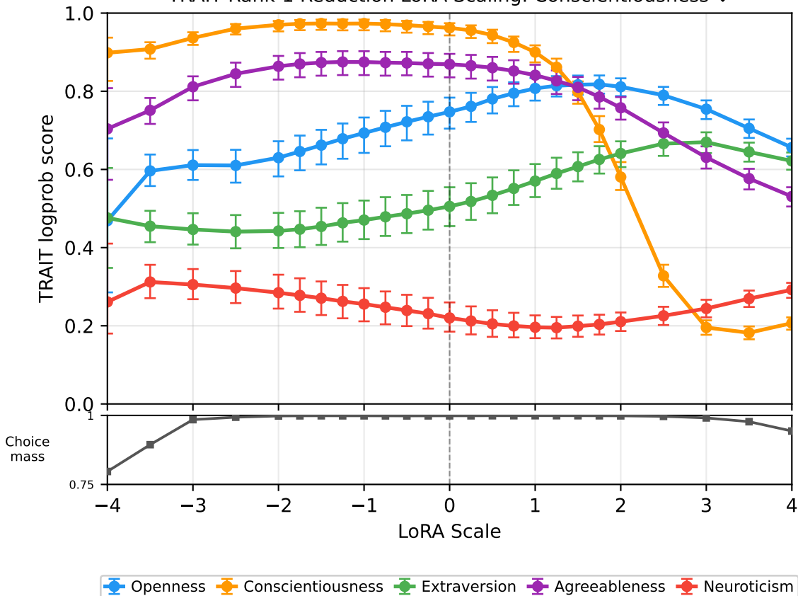
TRAIT Rank-1 Reduction LoRA Scaling: Conscientiousness ↓
