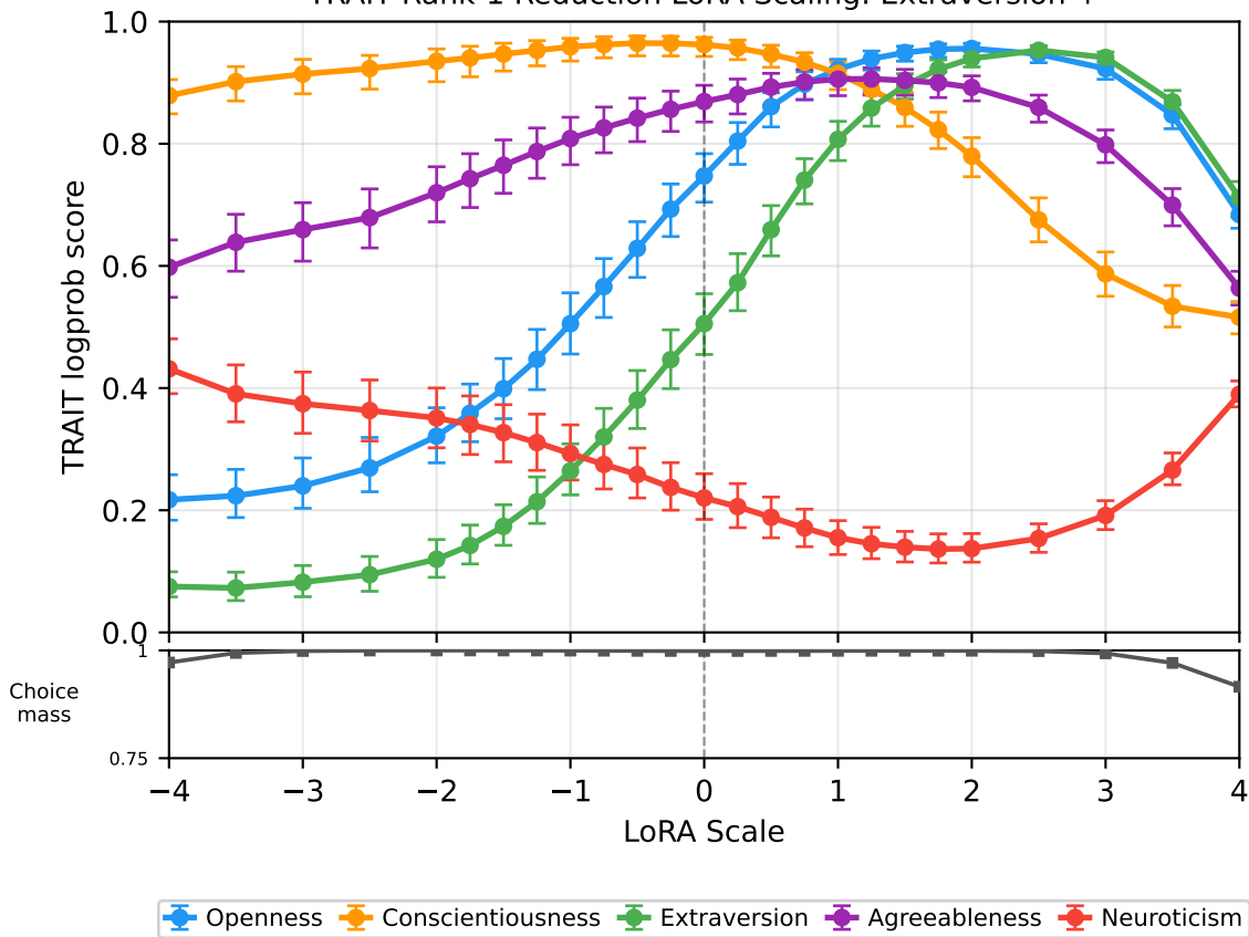
TRAIT Rank-1 Reduction LoRA Scaling: Extraversion \uparrow
