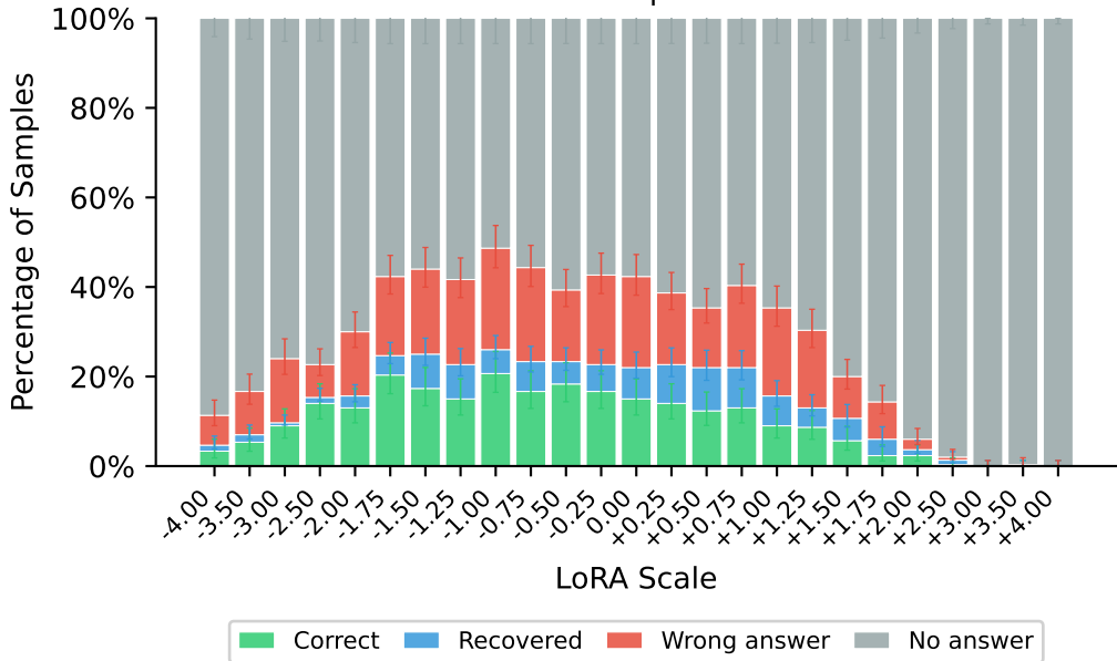
MMLU Base \leftrightarrow Instruct Interpolation: C \downarrow at w = 0.05
