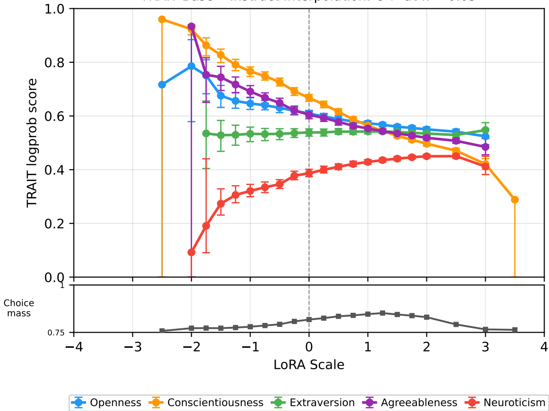
TRAIT Base \leftrightarrow Instruct Interpolation: C \downarrow at w = 0.05
