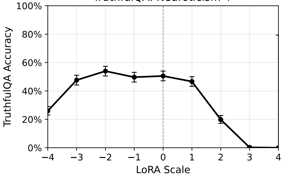
TruthfulQA: Neuroticism \uparrow
