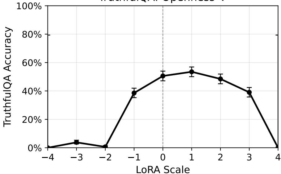
TruthfulQA: Openness ↓
