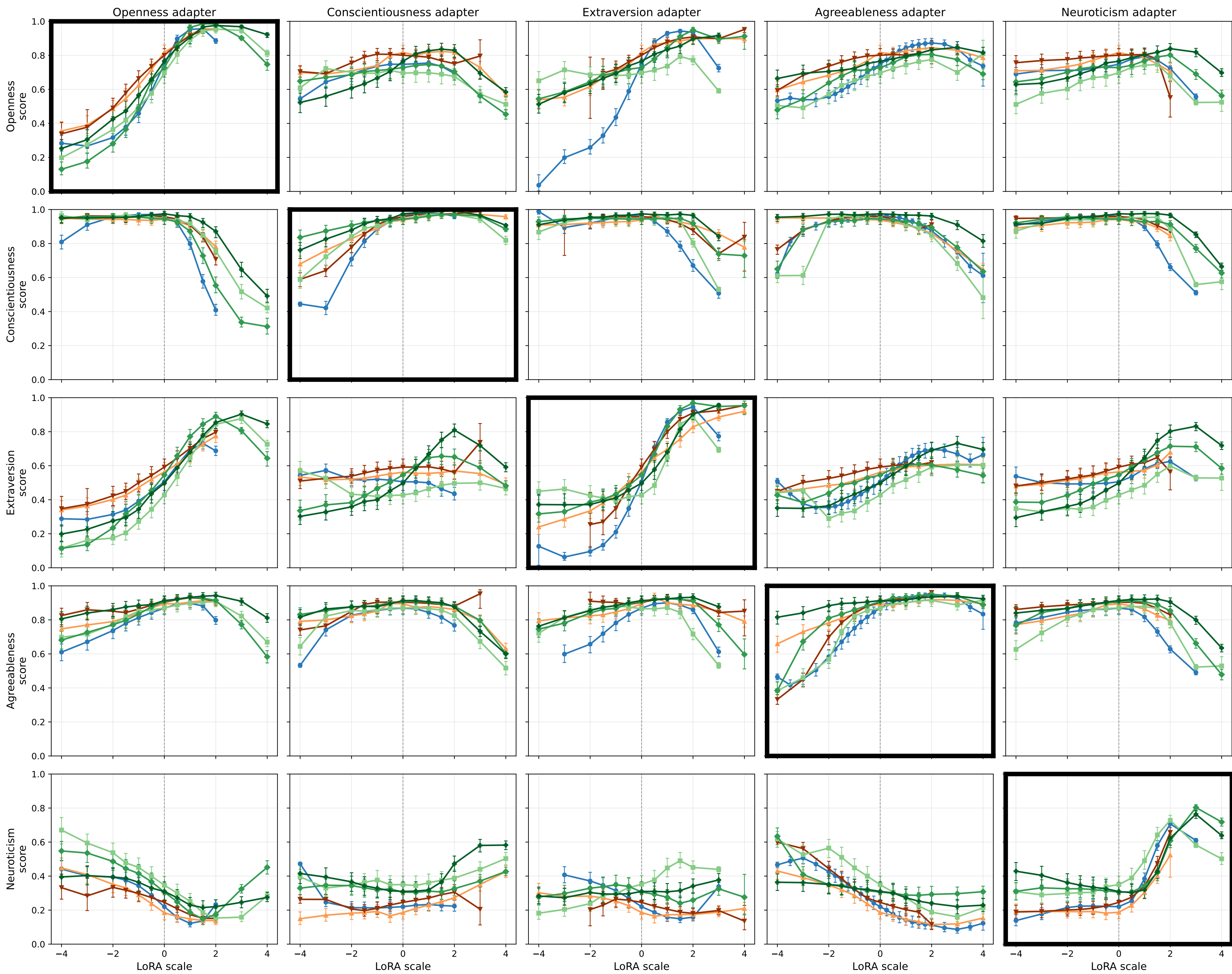
OCEAN amplifier adapters ↑ — applied adapter (columns) vs measured trait (rows); bold = on-target diagonal
