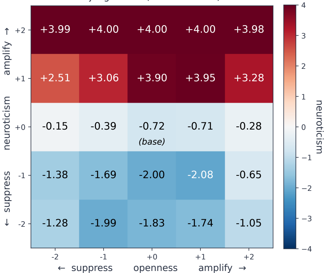
Neuroticism judge score (Gemma-3-12B)
