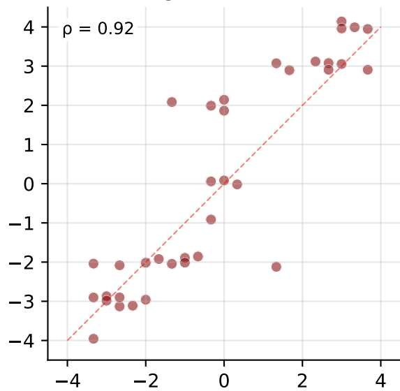
Agreeableness
