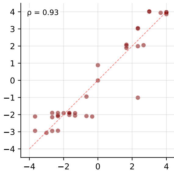
Neuroticism
