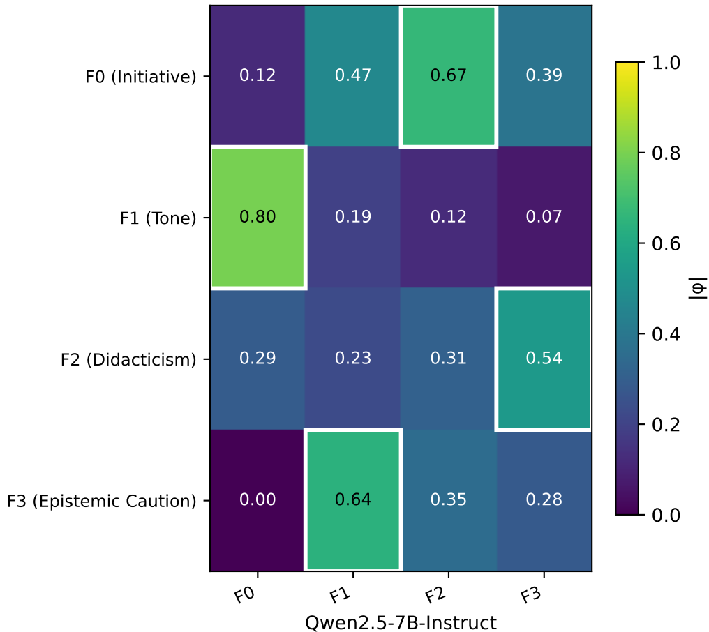
Tucker's |\phi| (combined, n_shared=53)
