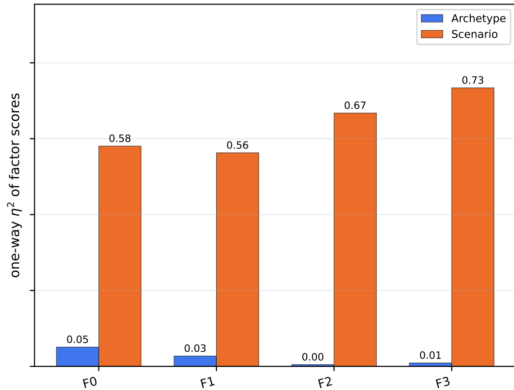
Qwen2.5-7B-Instruct
