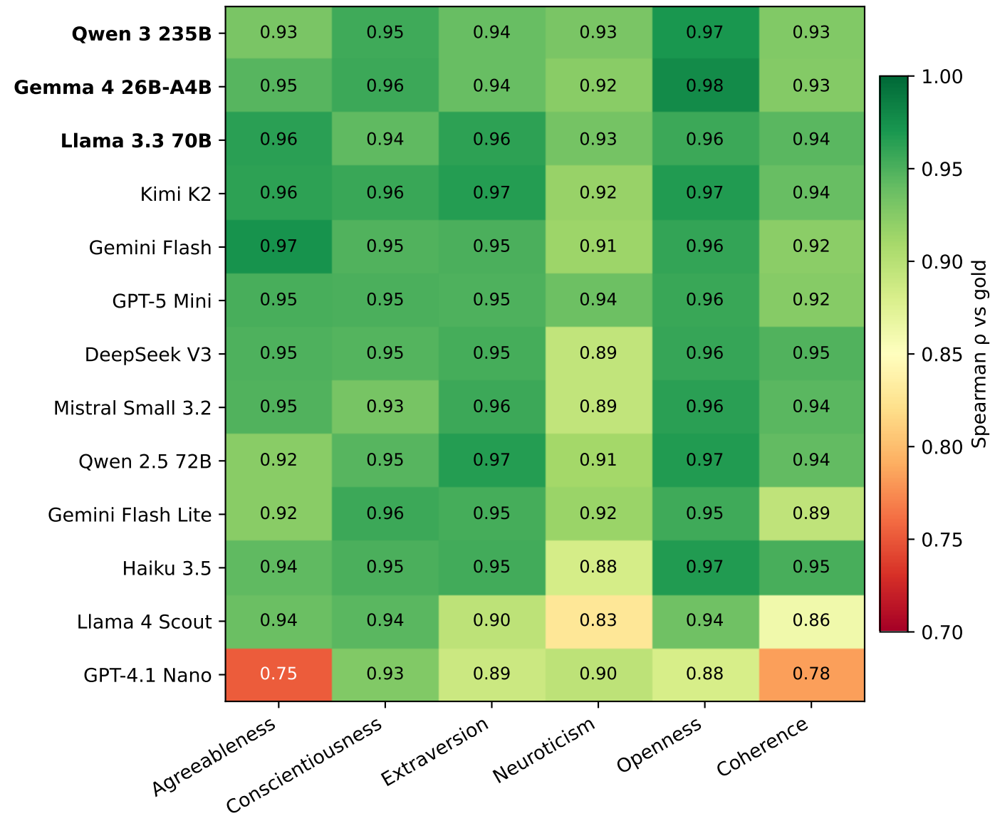
(a) Spearman \rho
