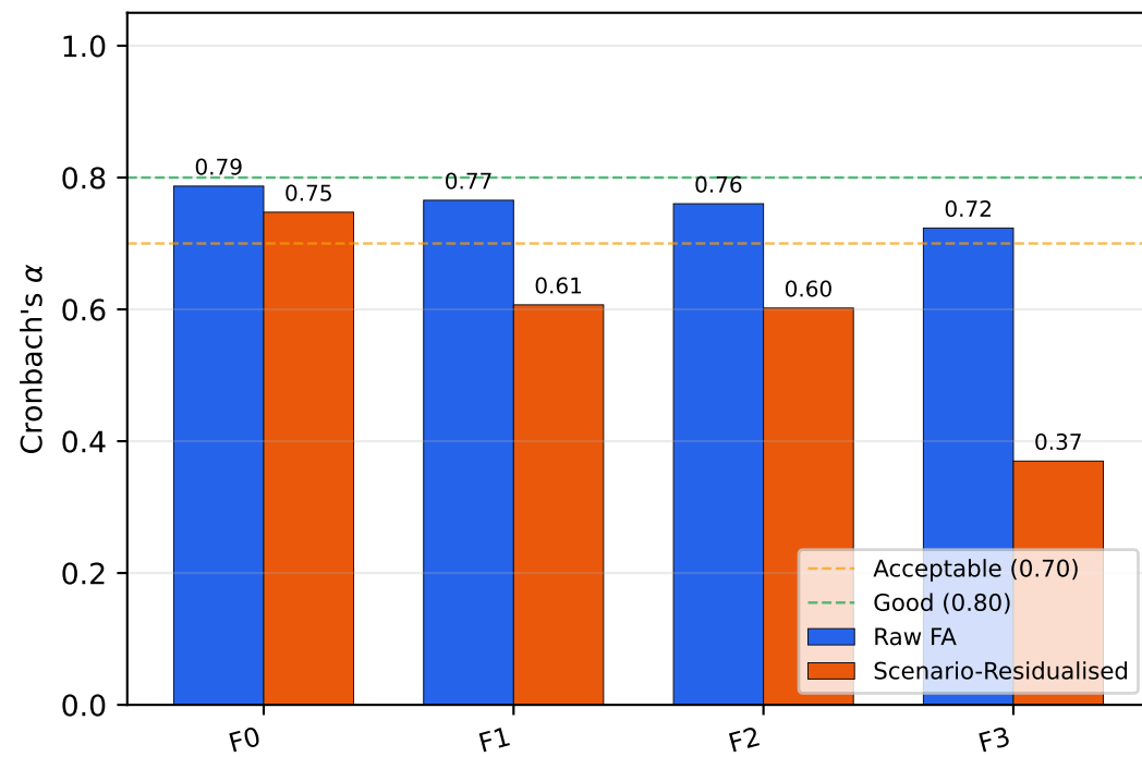
Qwen2.5-7B-Instruct: \alpha Before and After Scenario-Residualisation
