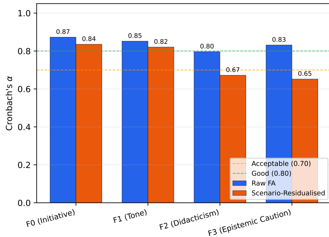
Qwen2.5-7B-Instruct: \alpha Before and After Scenario-Residualisation
