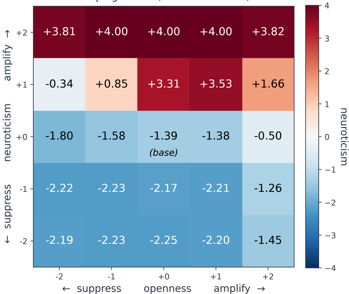
Neuroticism judge score (Gemma-3-27B-IT)
