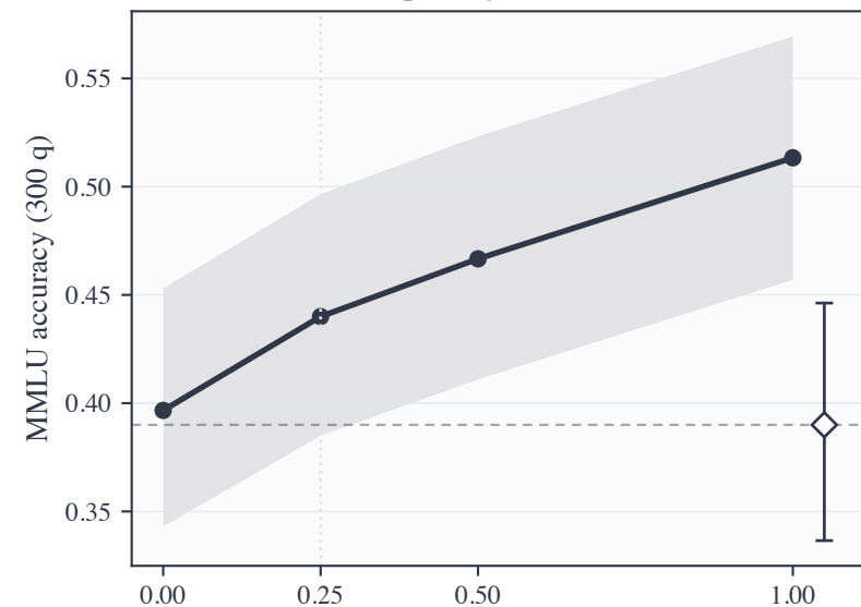
Capability (MMLU)
