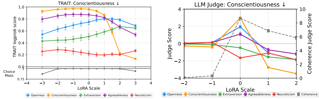
Figure 23: Conscientiousness \downarrow : TRAIT logprob (left) and Qwen3-235B-A22B LLM-judge (right) sweeps. The judge plot also shows answer coherence on the secondary axis. Judge data is collected at x \in \{-2, -1, 0, +1, +2\} . All error bars are 95% BCa bootstrap (1000 resamples) confidence intervals.
