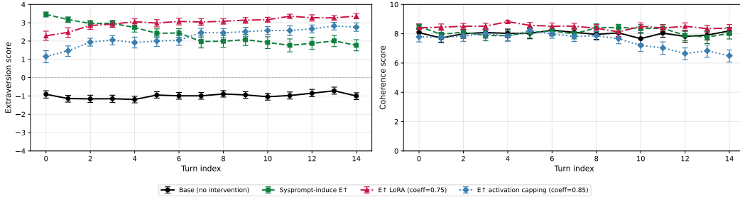
Figure 60: Per-turn extraversion (left) and coherence (right) trajectories for the four E↑ induction methods on neutral psychometric prompts. Each cell is 40 prompts \times 3 rollouts \times 15 turns (1800 assistant messages). Llama-3.1-8B-Instruct as assistant at temperature 0.7; GPT-4.1 mini as the user-simulator. Error bars show bootstrap 95% CIs over the per-prompt \times per-rollout sample.
