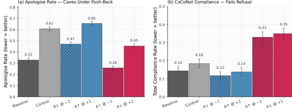
Figure 6: Sycophancy and compliance can be manipulated by varying agreeableness. Agreeableness raises sycophancy but lowers harmful compliance. (a) High-agreeableness conditions (A \uparrow at +1, A \downarrow at -1) capitulate more under "are you sure?" pressure than low-agreeableness conditions (A \uparrow at -1, A \downarrow at +1). (b) Low-agreeableness conditions comply when they should not 2.3x more frequently compared to baseline. Error bars are 95% Wilson CIs.
