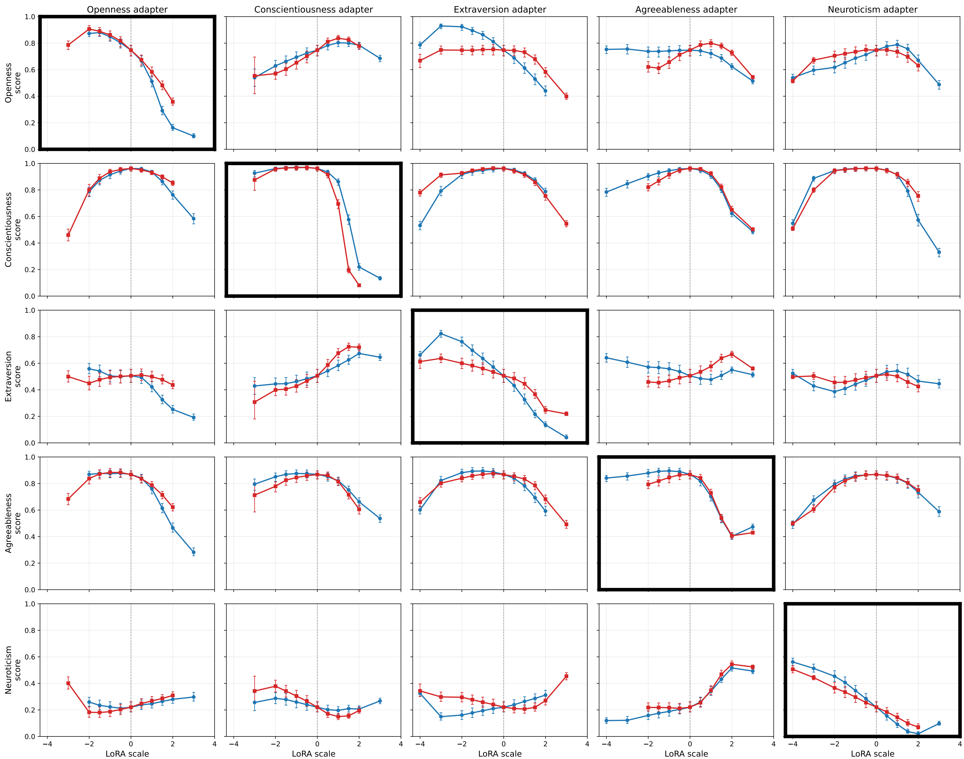
OCEAN suppressor adapters ↓ — applied adapter (columns) vs measured trait (rows); bold = on-target diagonal
