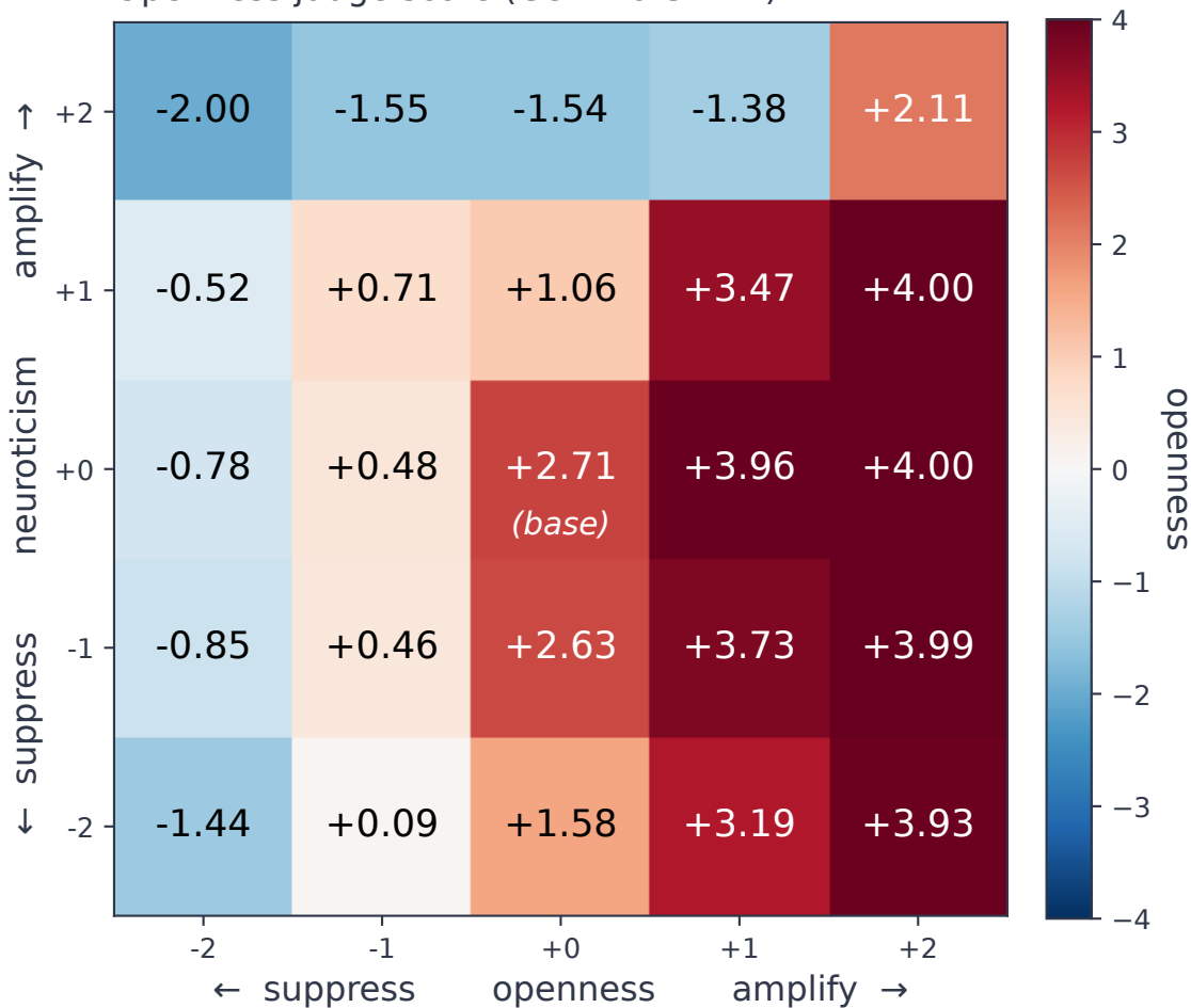
Openness judge score (Gemma-3-12B)
