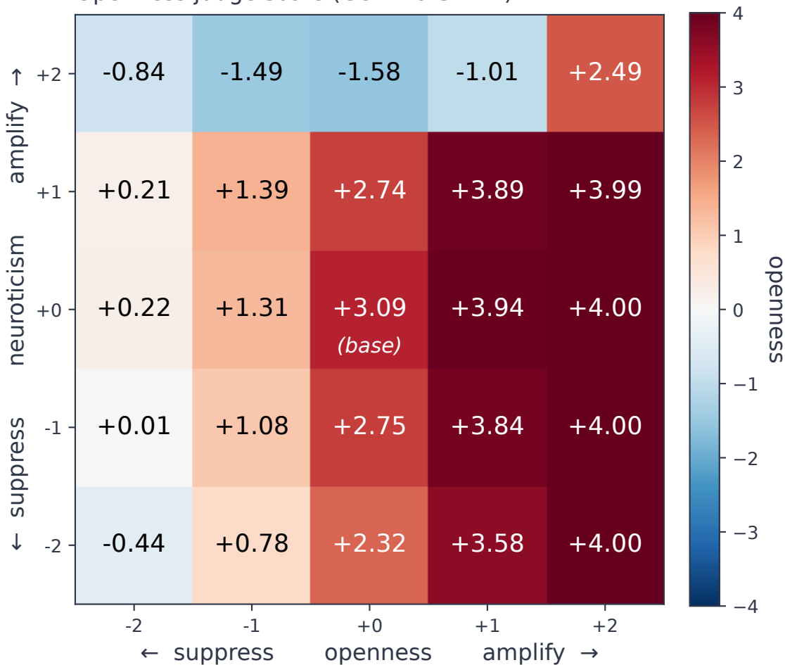
Openness judge score (Gemma-3-27B)
