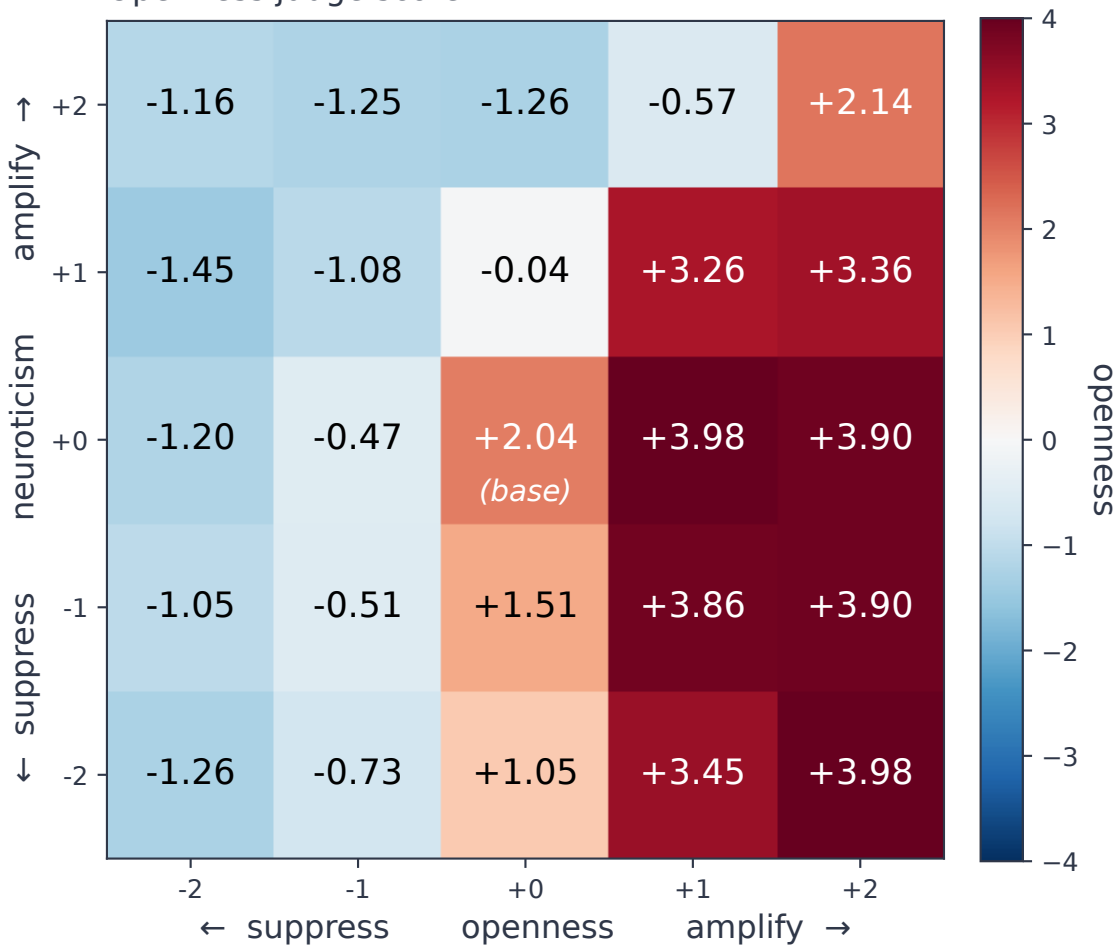
Openness judge score
