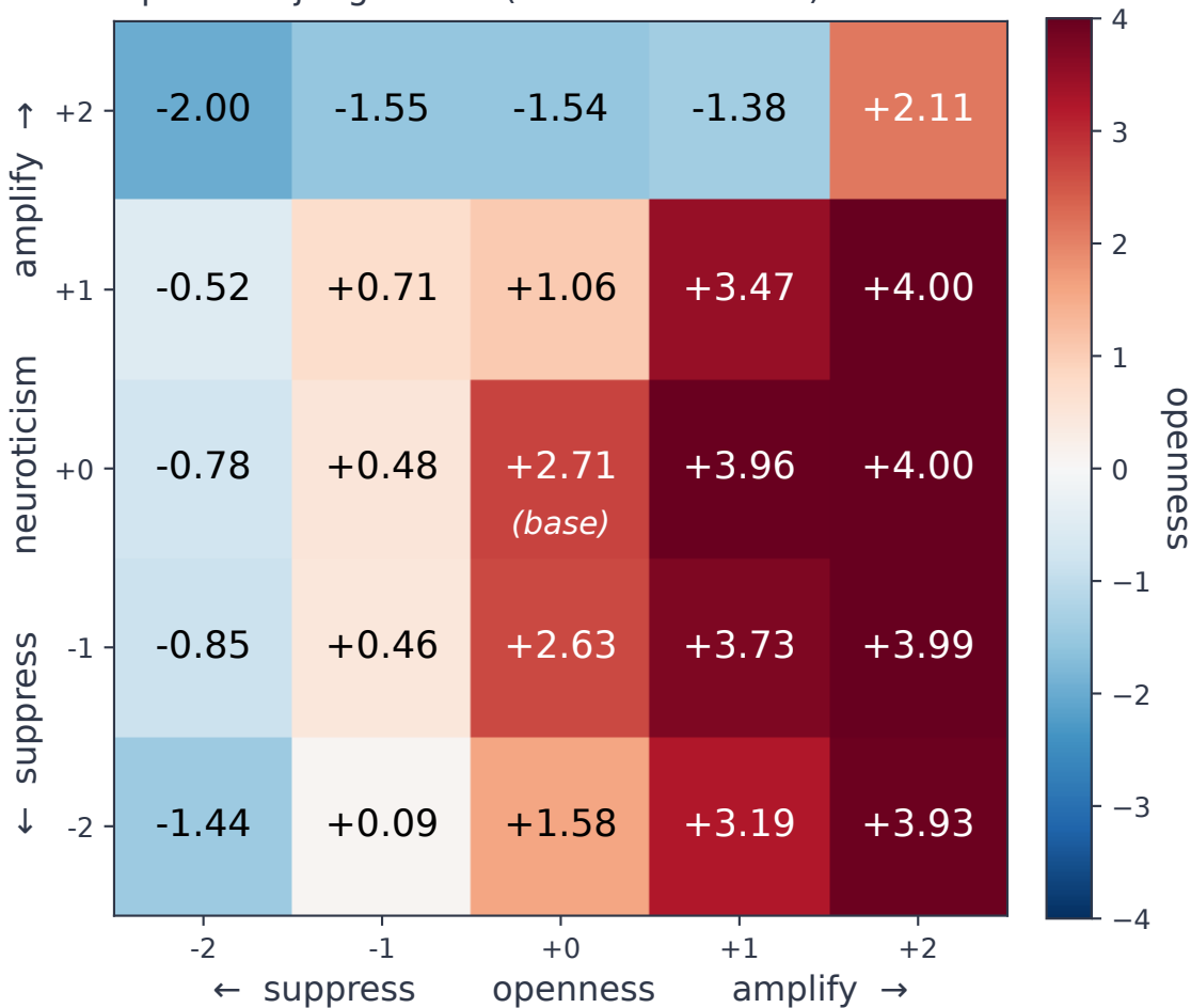
Openness judge score (Gemma-3-12B-IT)
