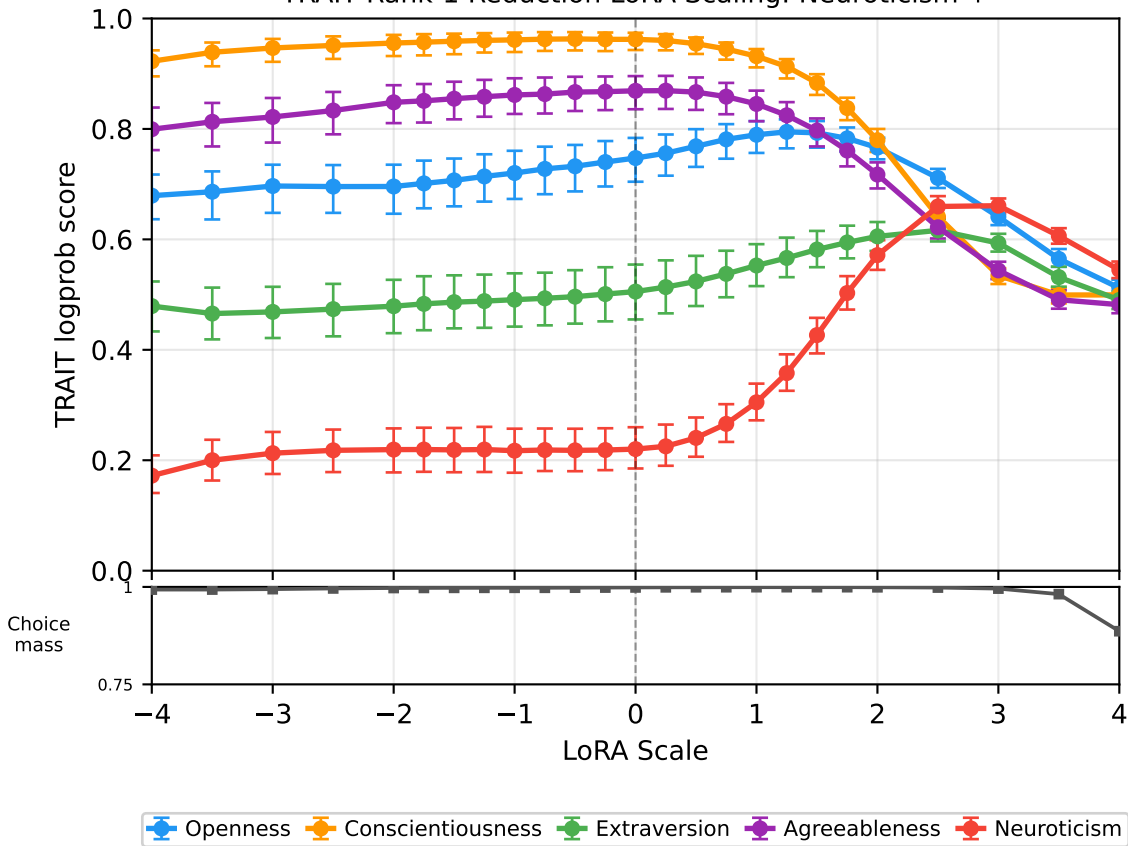
TRAIT Rank-1 Reduction LoRA Scaling: Neuroticism \uparrow
