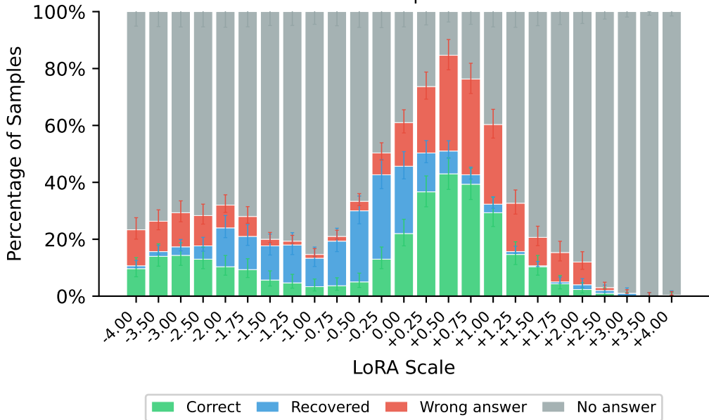
MMLU Base \leftrightarrow Instruct Interpolation: C \downarrow at w = 0.25
