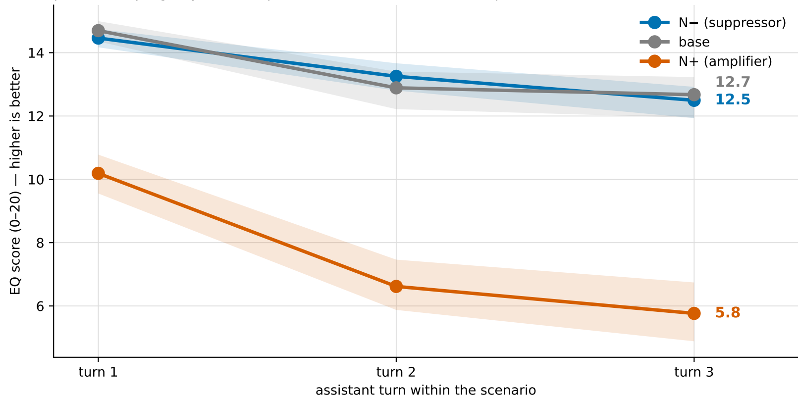
EQ across a multi-turn conversation — gemma-3-27b-it neuroticism adapters per-turn re-judge by claude-opus-4-6; bands = 95% bootstrap CI (n=44/turn/variant)
