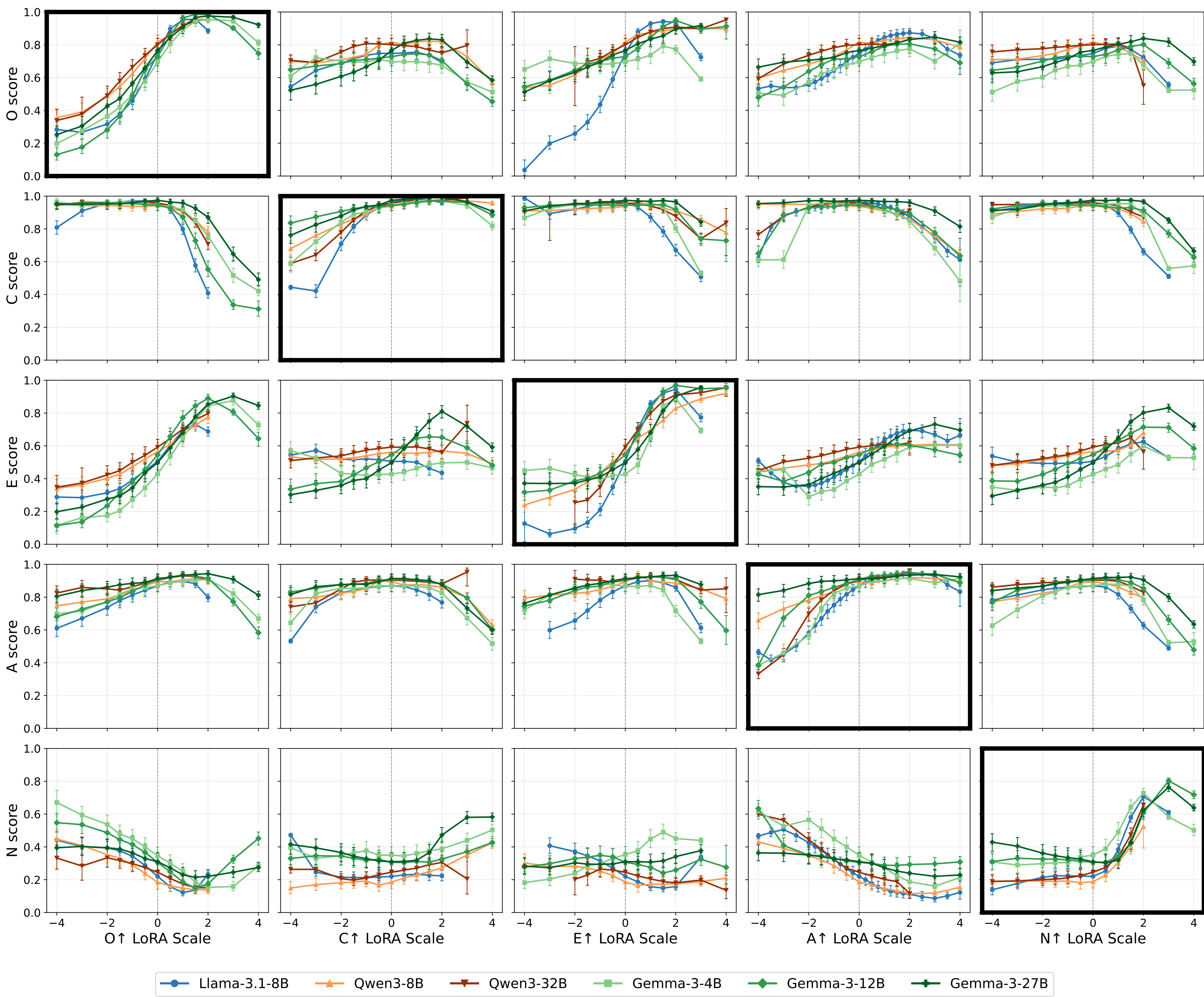
Model Comparison: OCEAN Trait Scores vs LoRA-Scale Sweep - Amplifier Adapters
