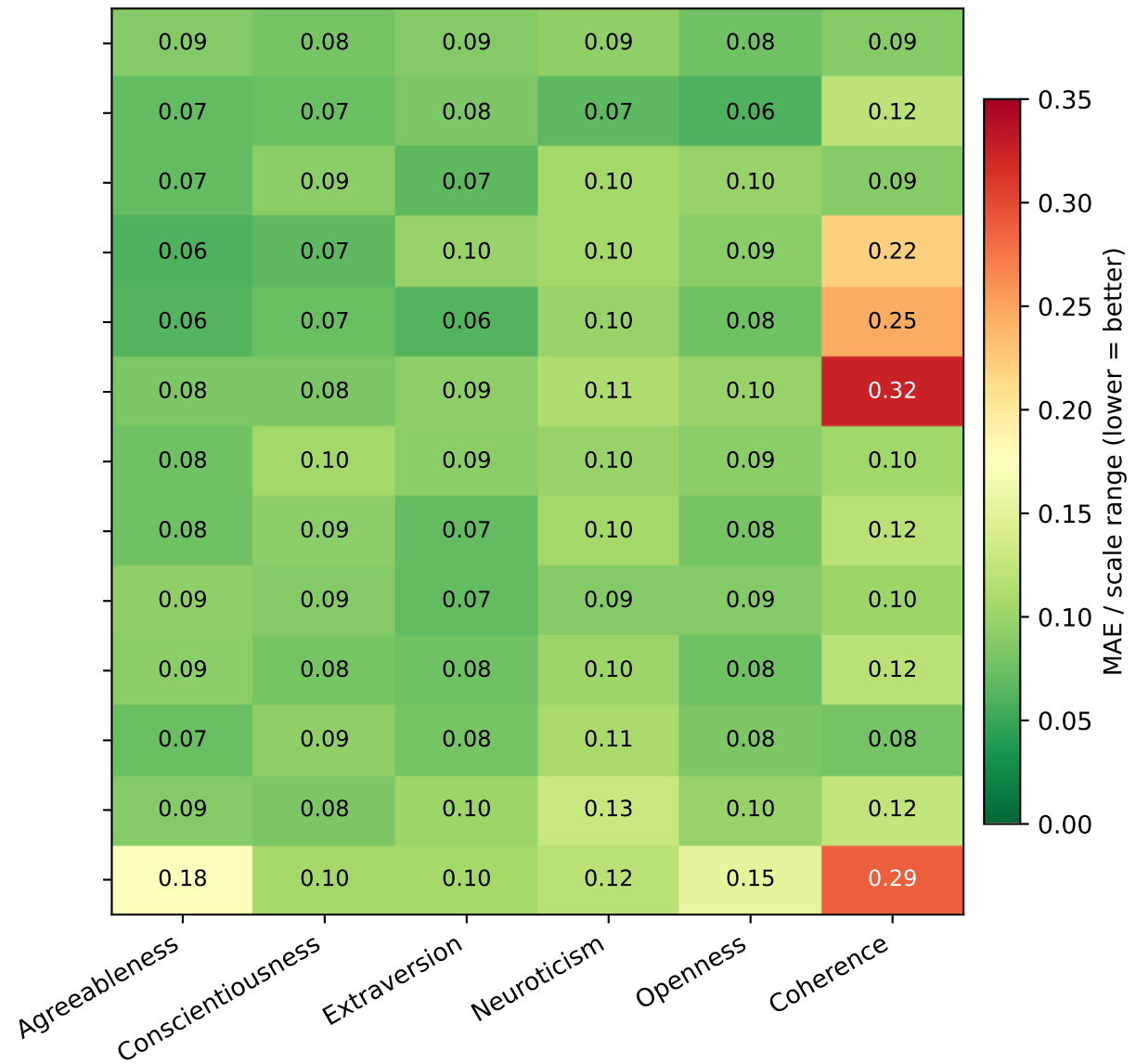
(b) Normalised MAE
