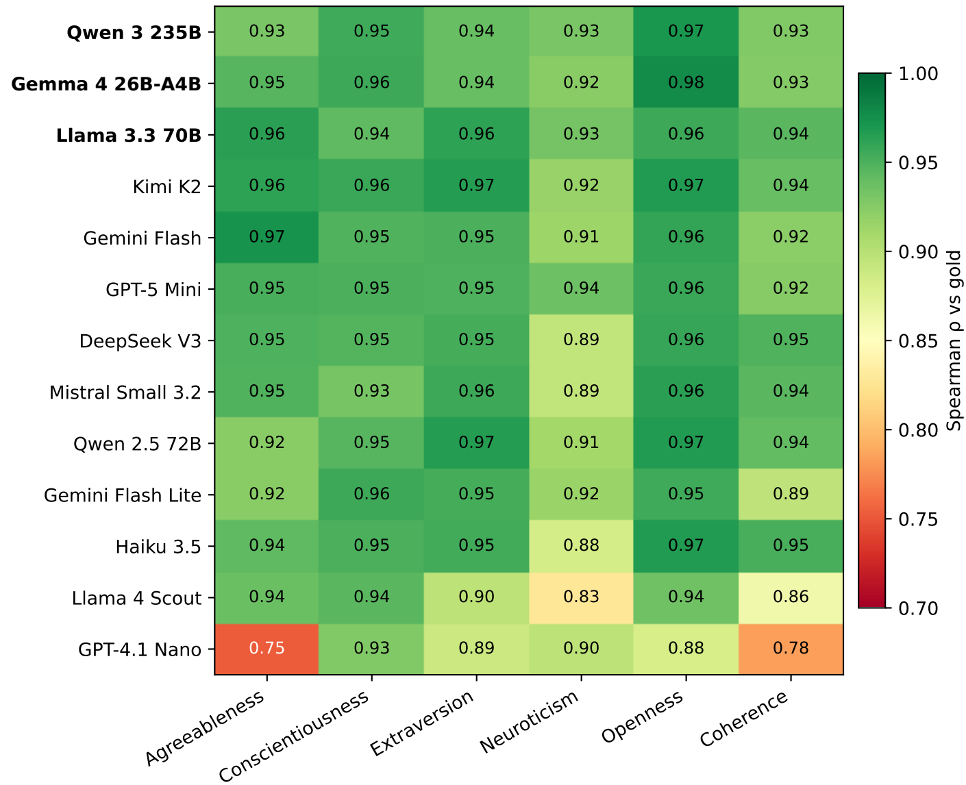
(a) Spearman \rho
