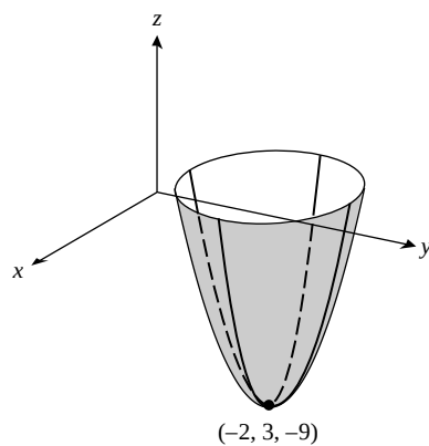
37. Circular paraboloid
