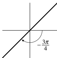
22. Line
