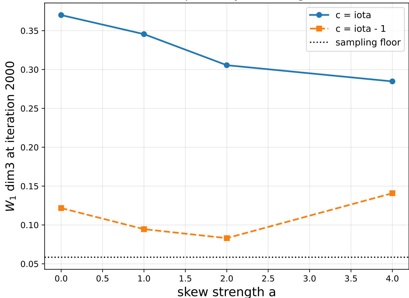
Anisotropic heavy-tailed target
