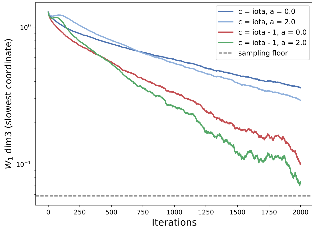
Anchor and J compose
