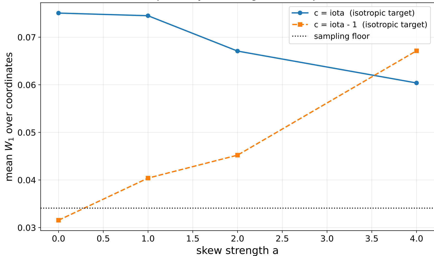
Isotropic heavy-tailed target: little for J to do
