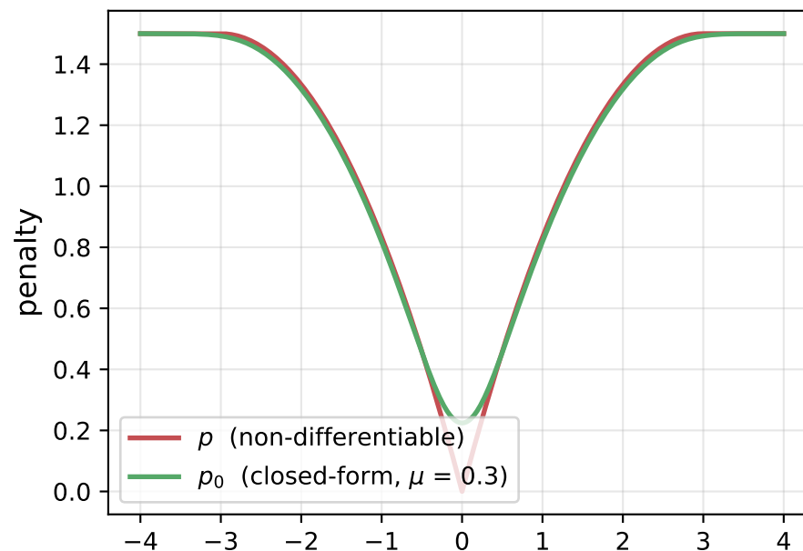
MCP
