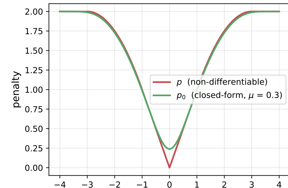
SCAD
