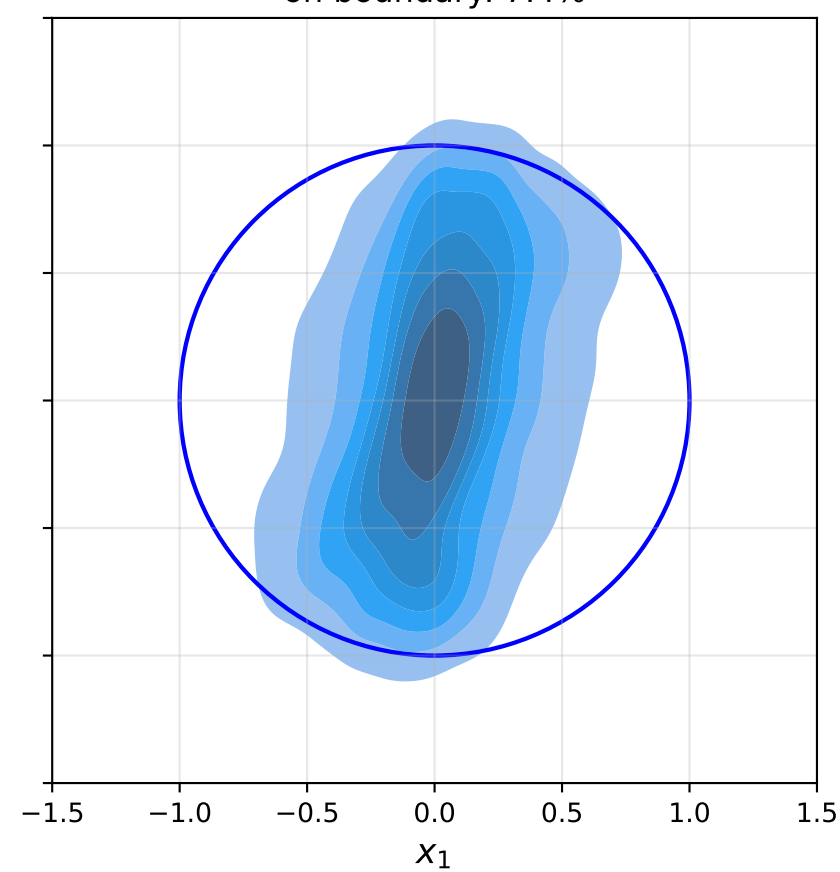
constant J_a , a = 4.0 on boundary: 7.4%
