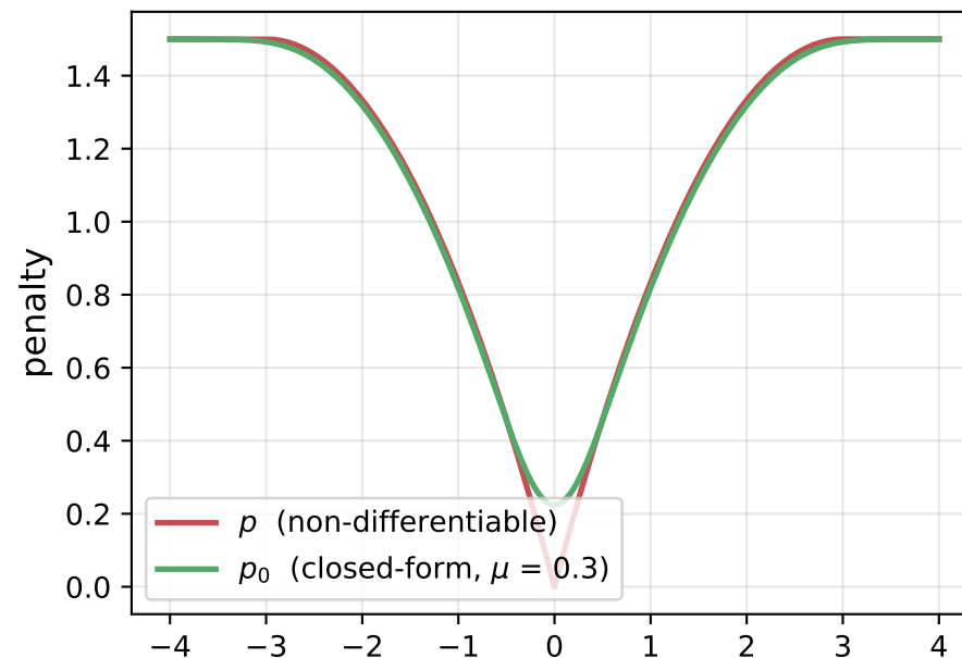
MCP
