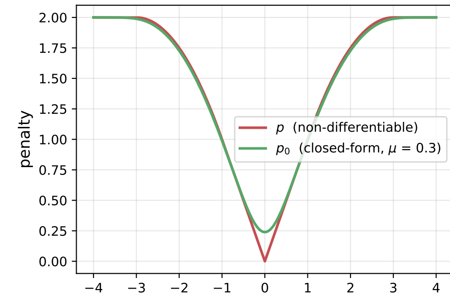
SCAD
