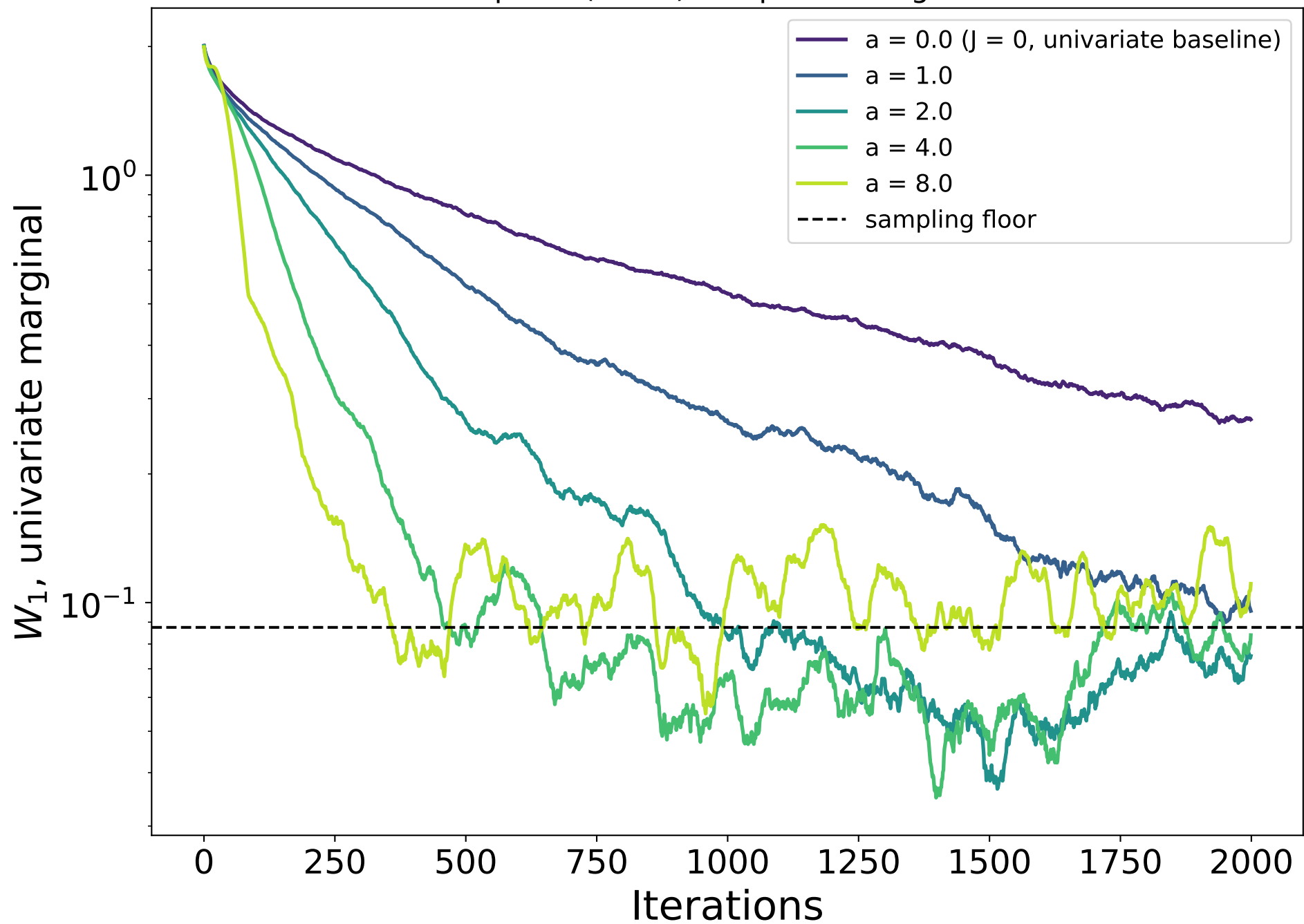
Univariate Laplace ( b = 2 ) sampled through a 2D skew lift
