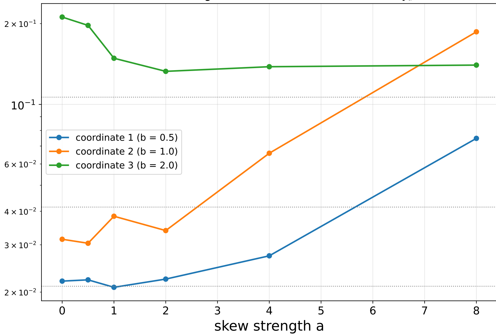
Anchored Langevin: effect of the constant skew J_a
