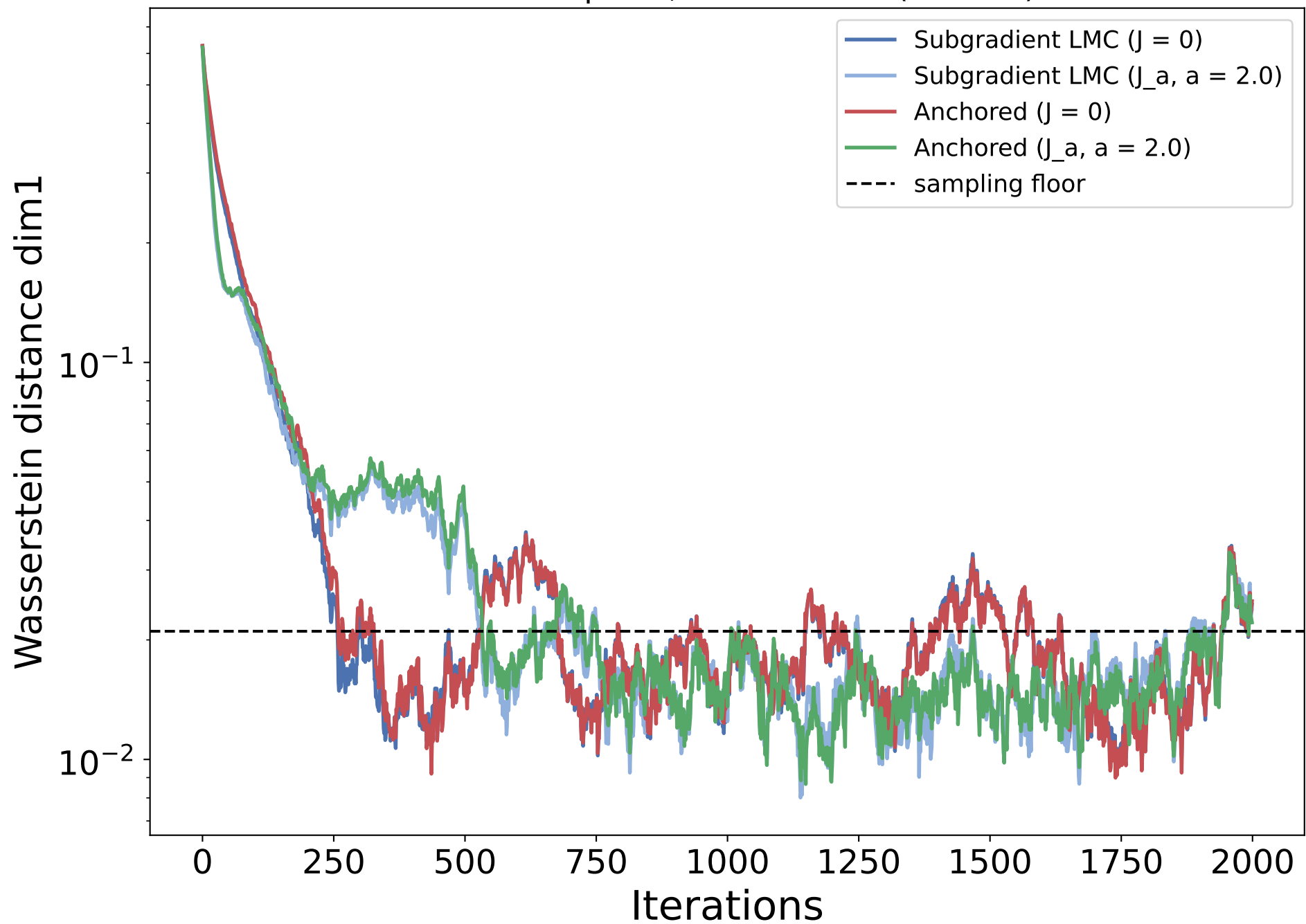
Product Laplace, coordinate 1 ( b = 0.5 )
