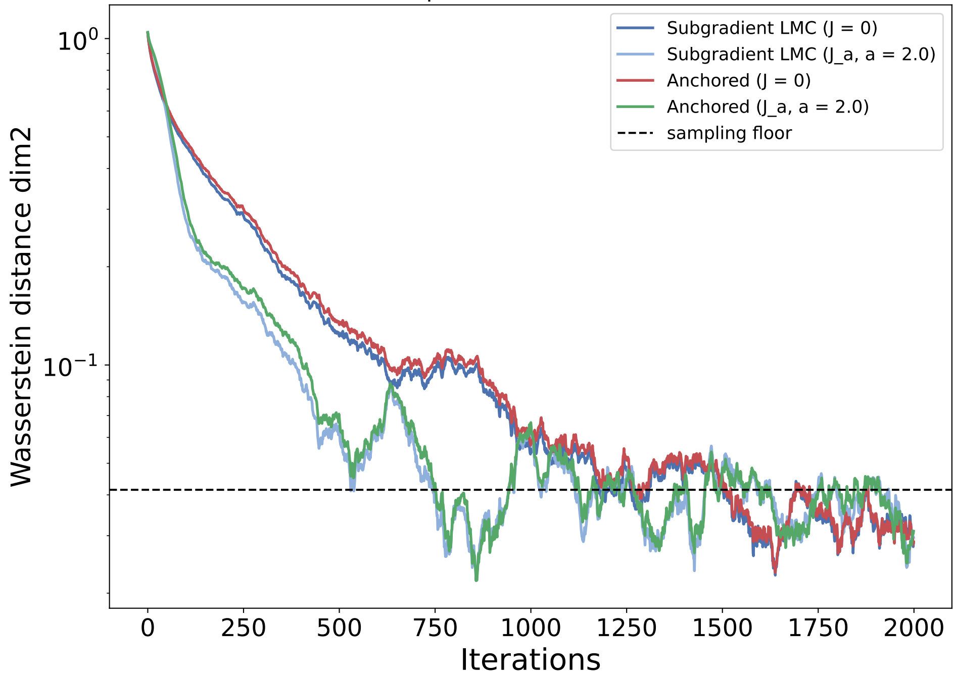
Product Laplace, coordinate 2 ( b = 1.0 )
